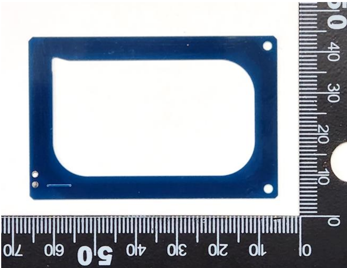
Bottom of 13.56 MHz Antenna
