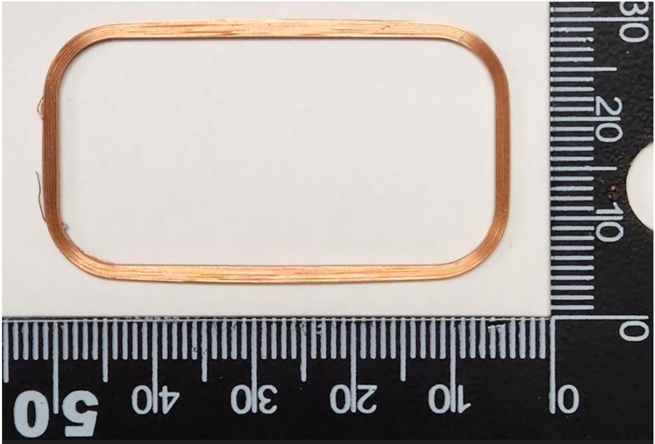
125 kHz Antenna
