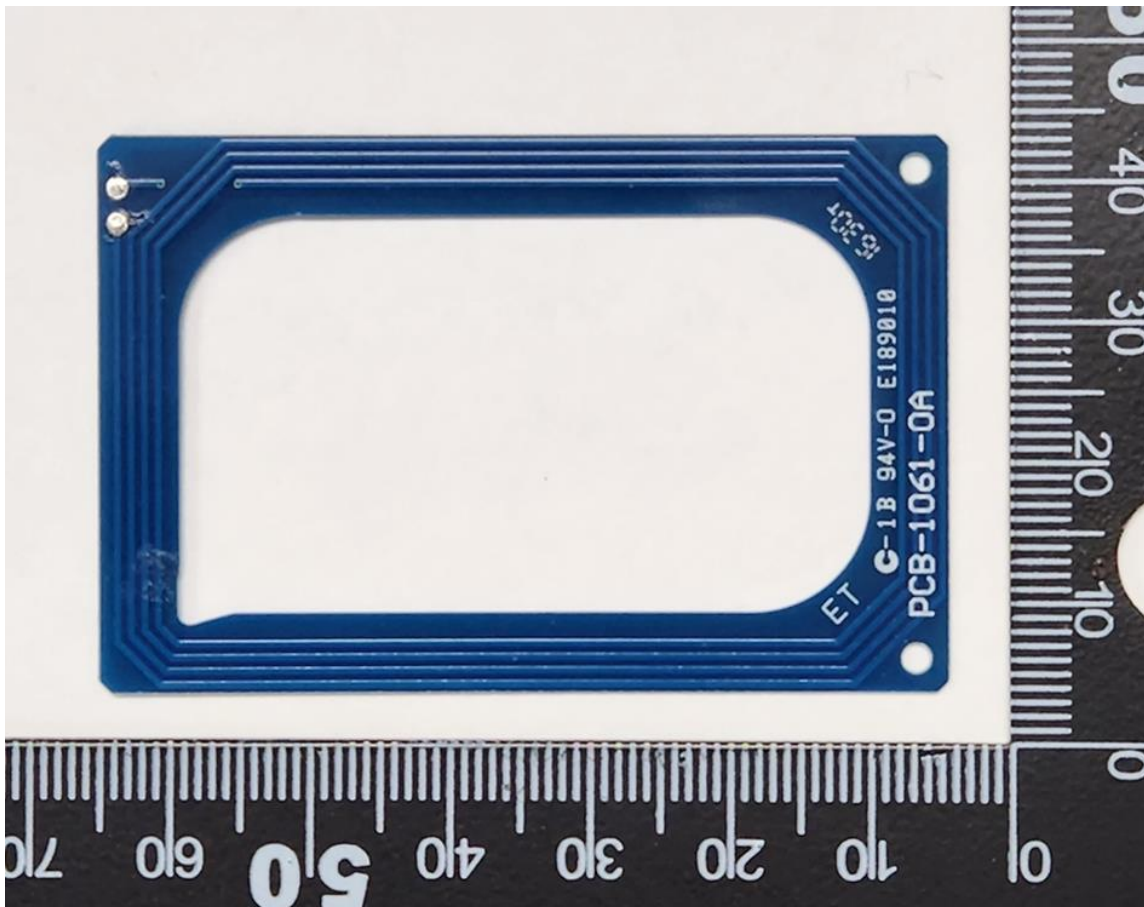
Top of 13.56 MHz Antenna
