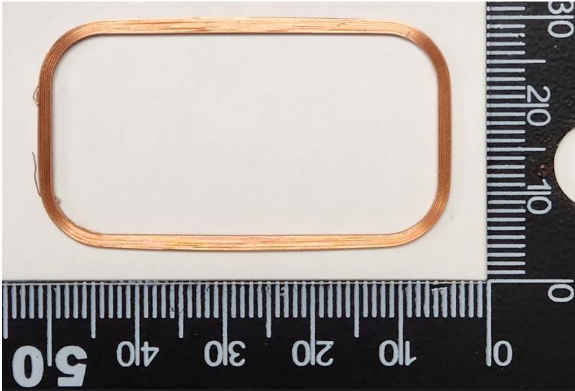
125 kHz Antenna
