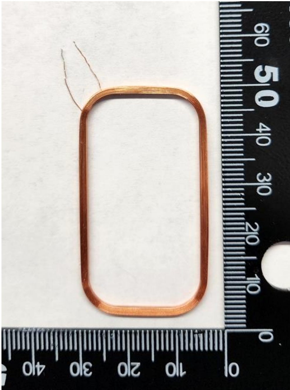
125 kHz Antenna
