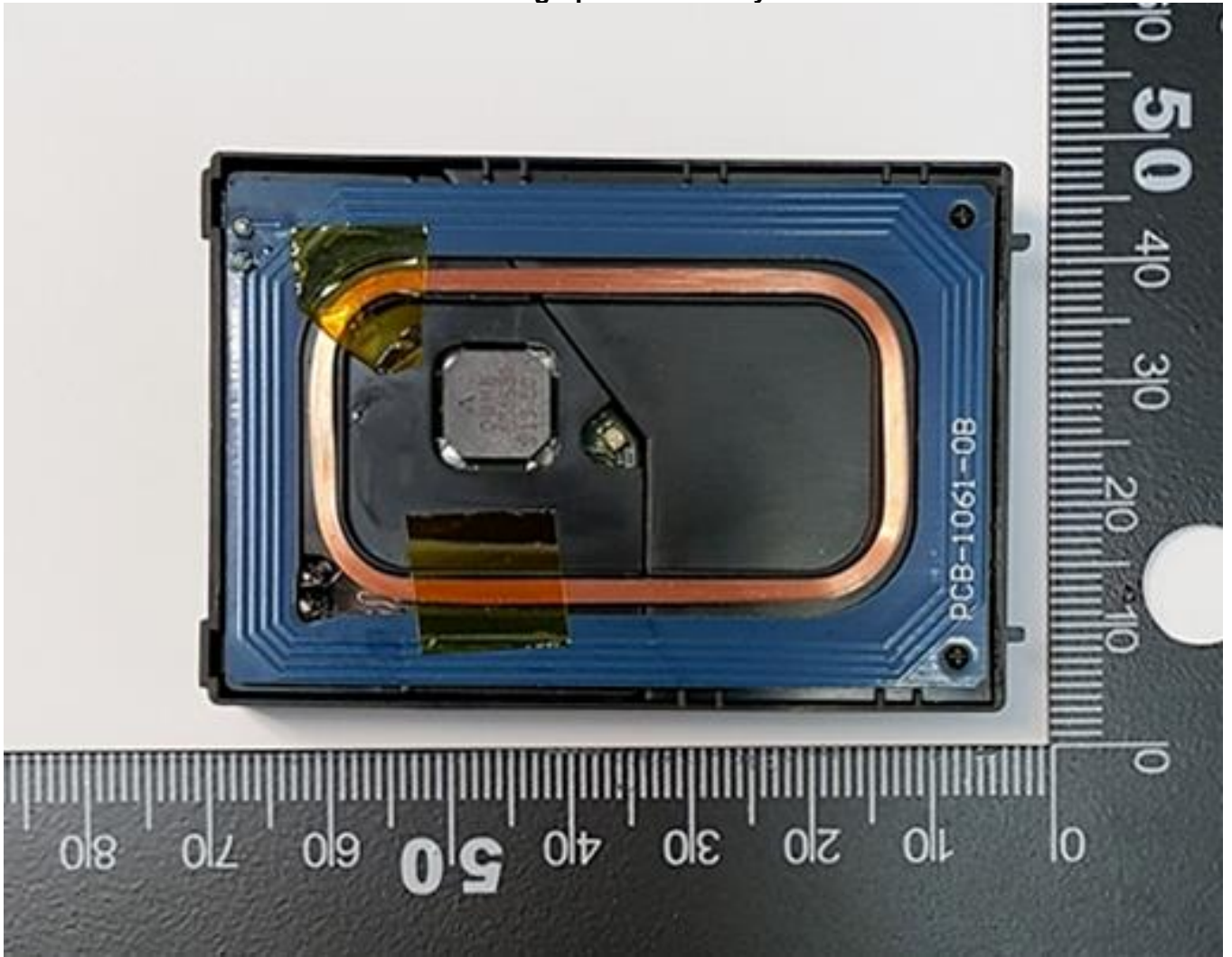
Photograph of assembly
