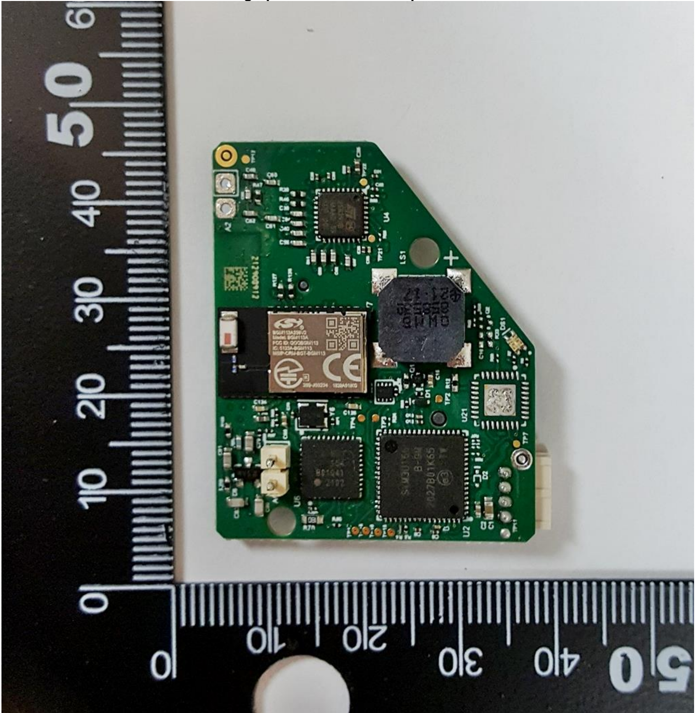
Photograph of PC Board: Component Side
