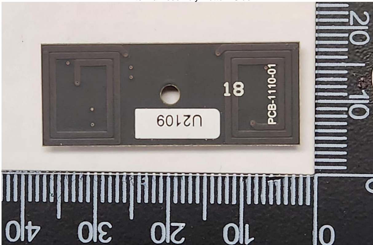
Antenna Assembly-Bottom Side
