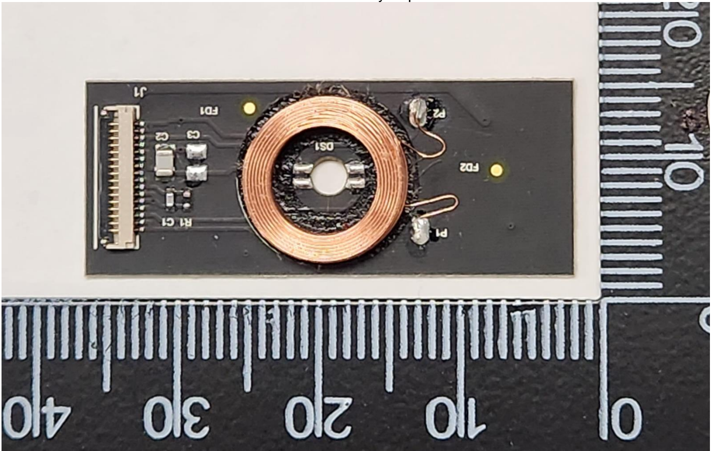
Antenna Assembly-Bottom Side
