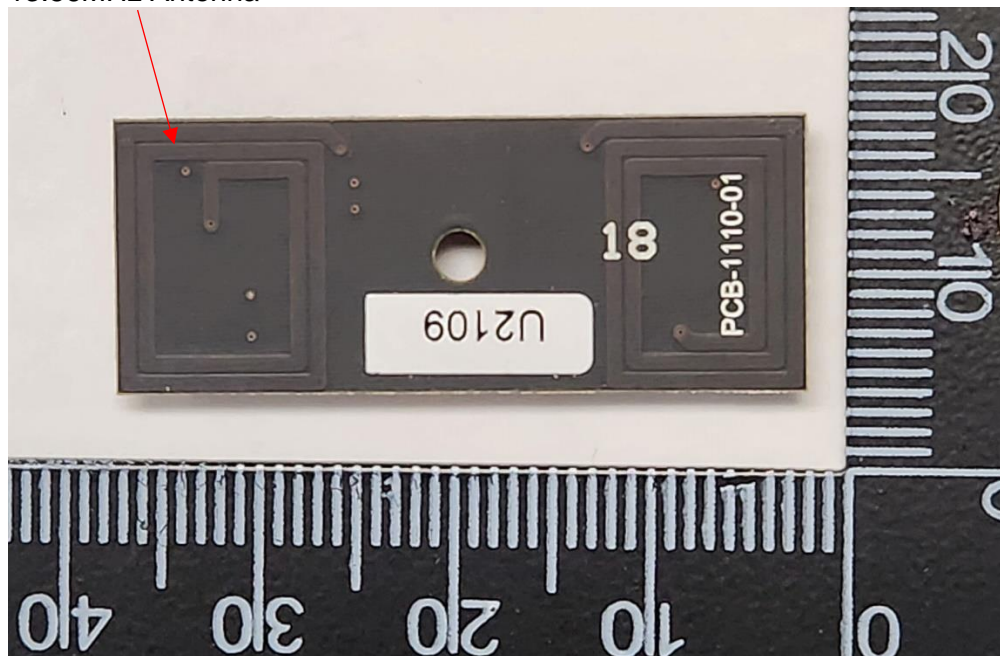
13.56MHz Antenna
