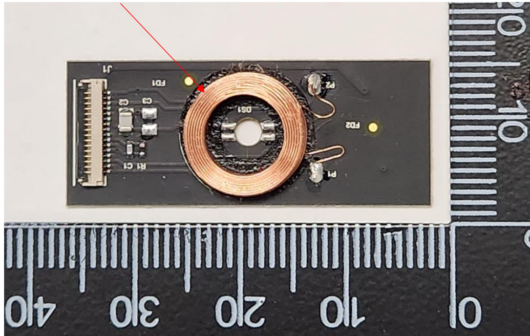
125 kHz Antenna
