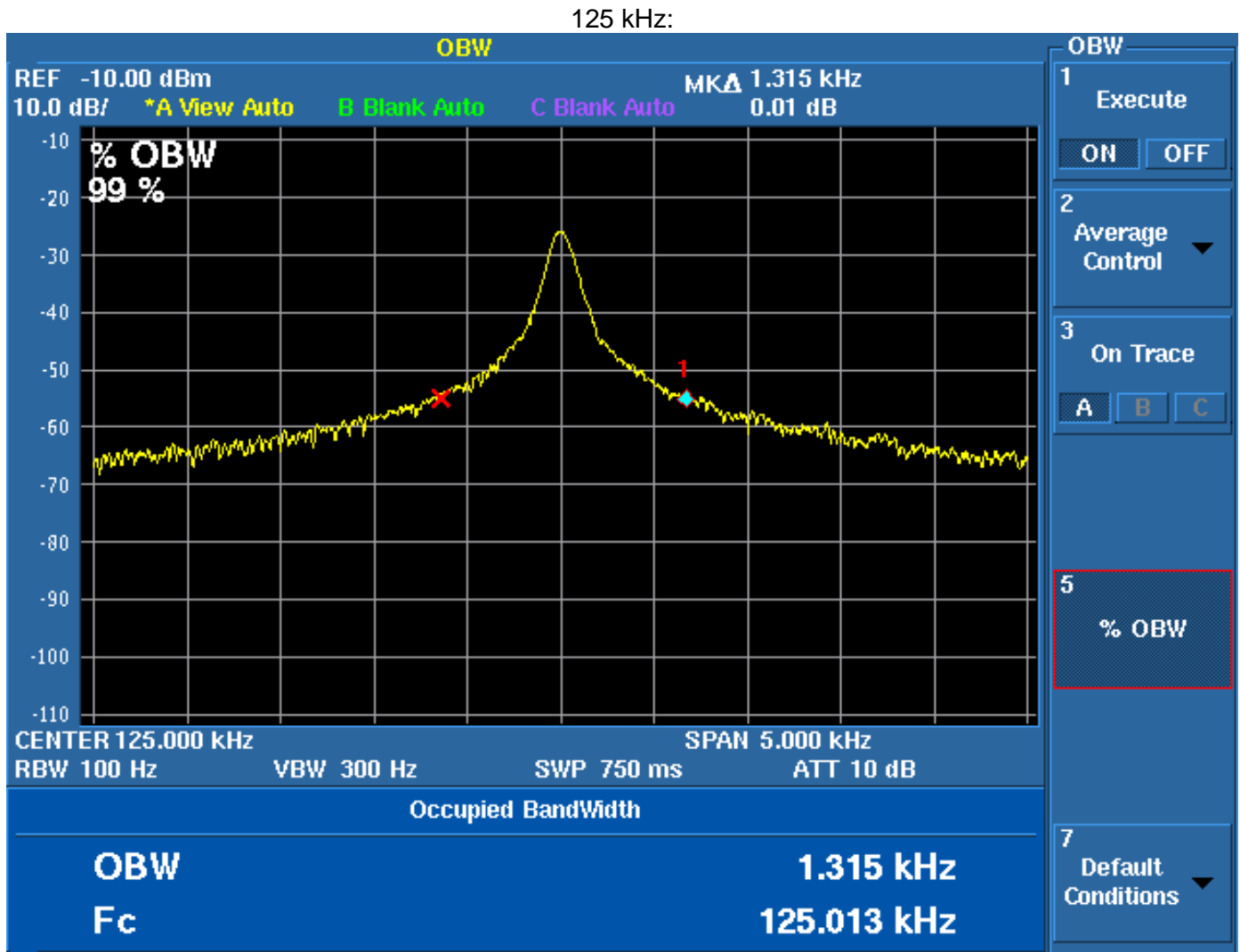
Figure 3. Occupied Bandwidth Plot
