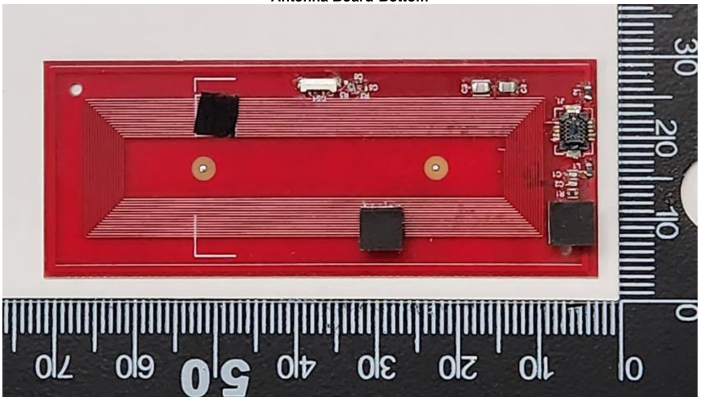
Antenna Board-Bottom
