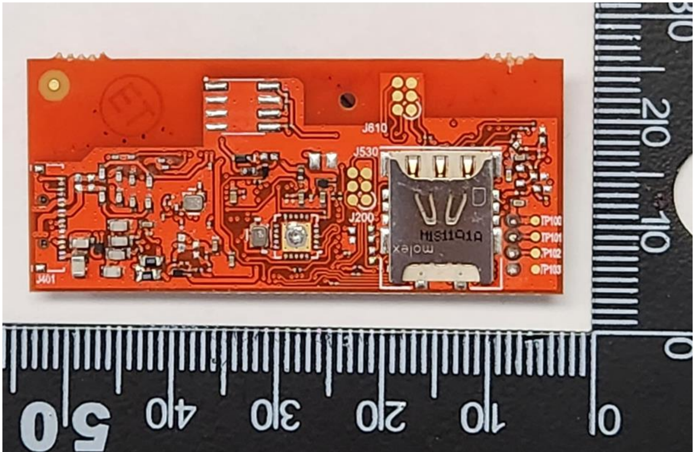
PC Board-Bottom
