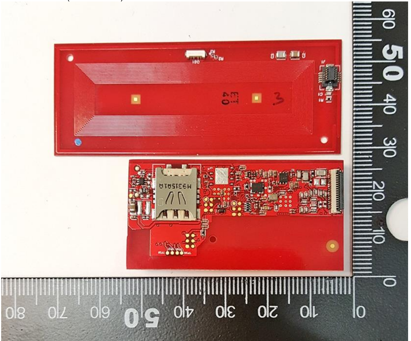
Model 30541AKU (Bottom Sides)
