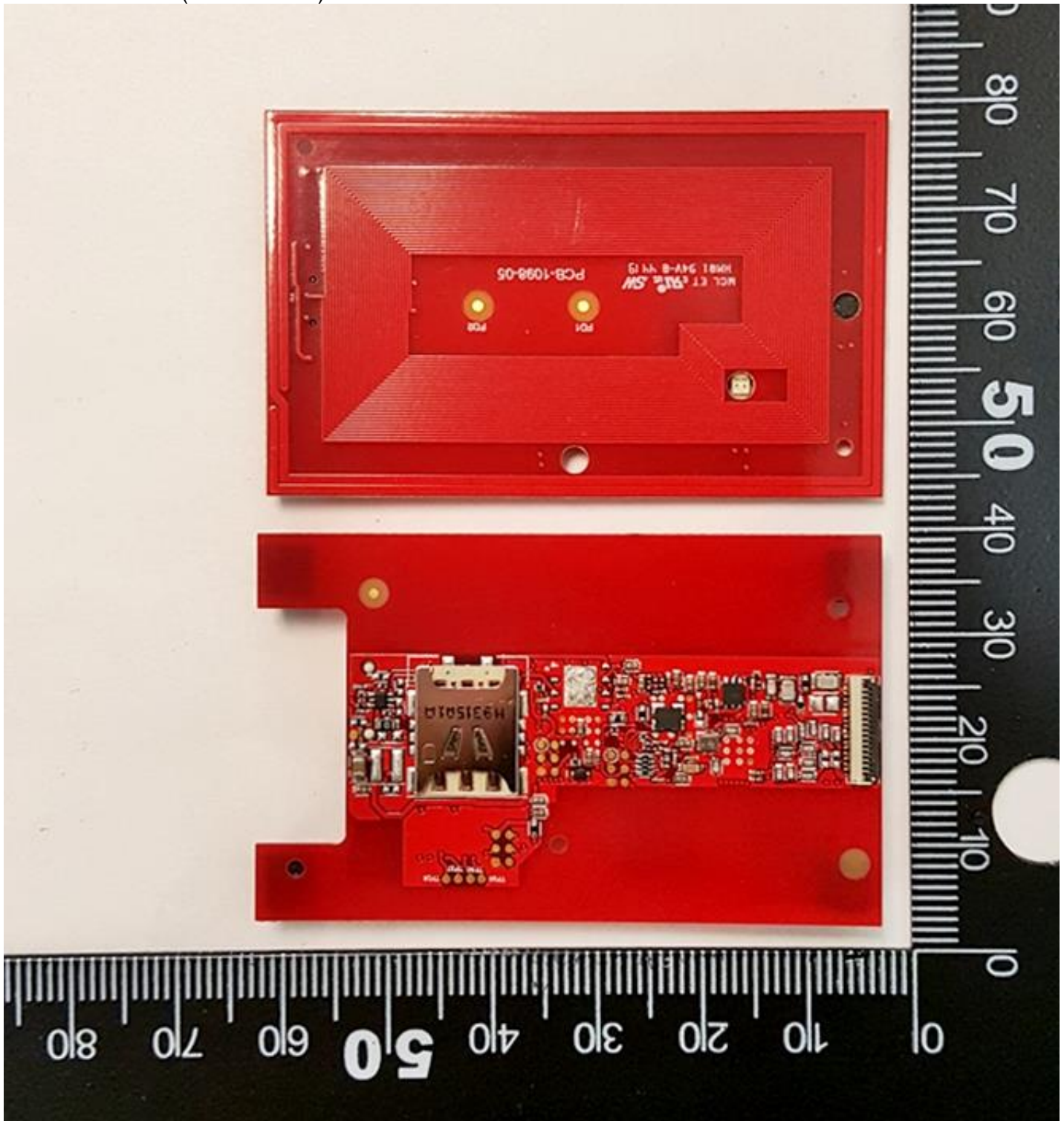
Model 30531AKU (Bottom Sides)
