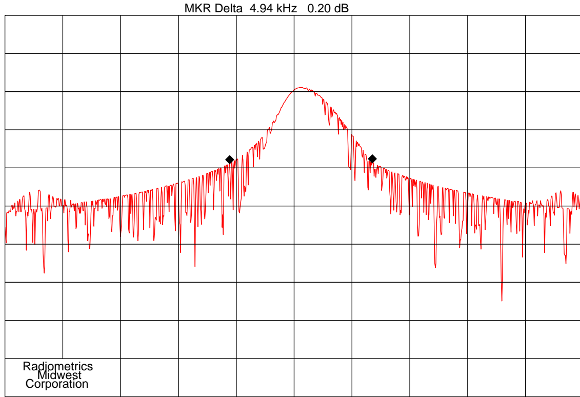
Figure 4. Occupied Bandwidth Plots 13.56 MHz
