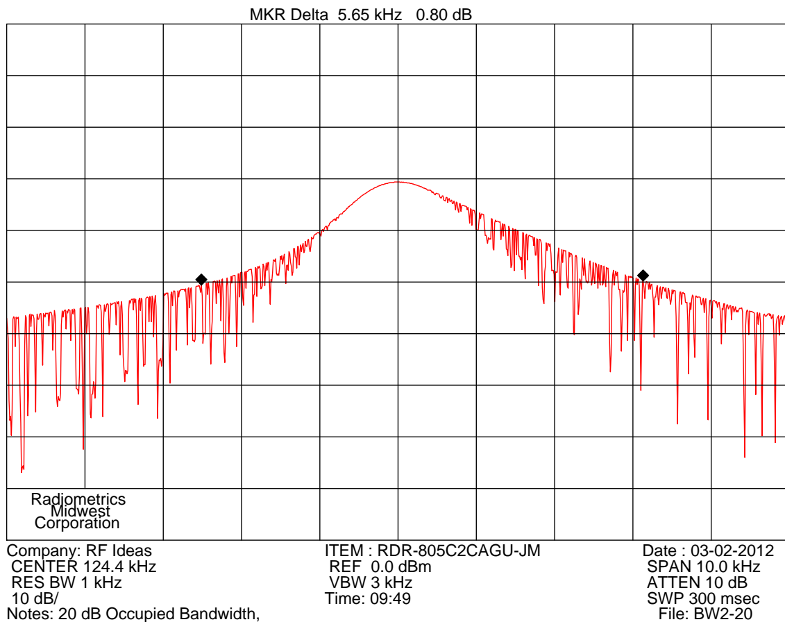
Figure 3. Occupied Bandwidth Plots 125 kHz
