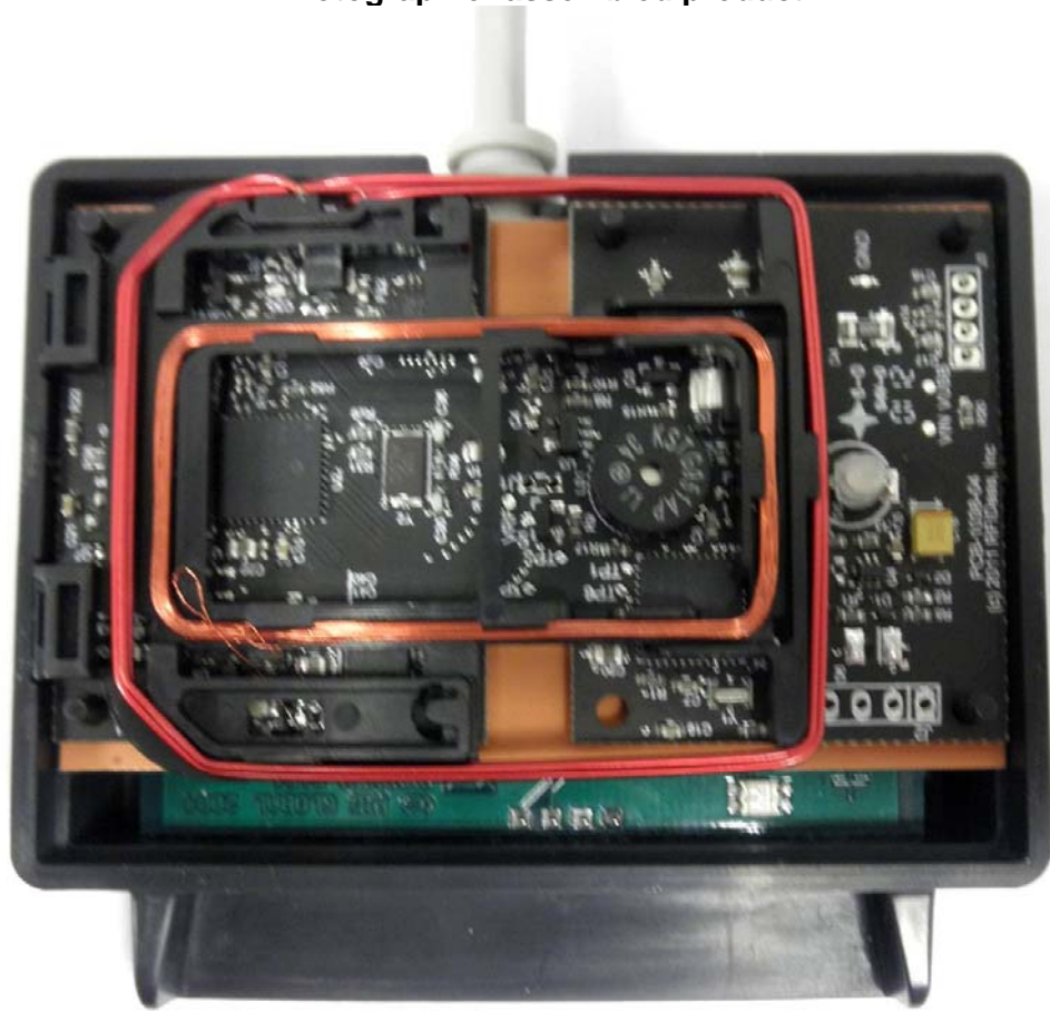
Photograph of assembled product
