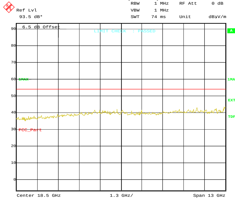
Plot : 12- 25 GHz vertical/horizontal (receiver)
