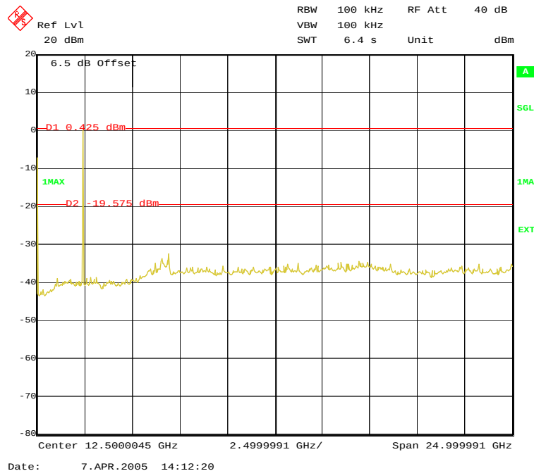
Plot 2 of 3: middle channel
