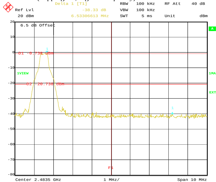
Plot 3 of 4 (hopping off, highest frequency):
