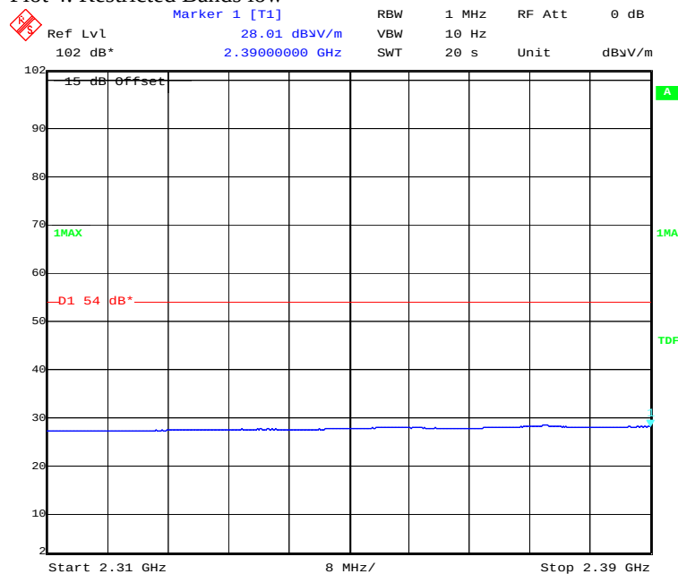
Plot 4: Restricted Bands low
