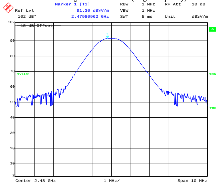
Plot 1 : Max field strength in 3m distance (single frequency)
