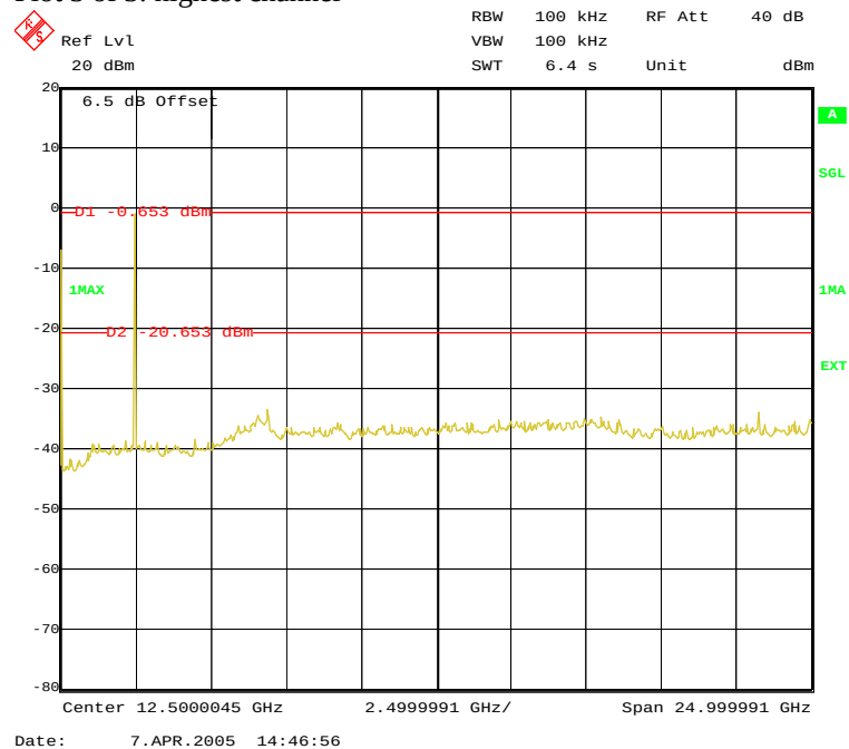
Plot 3 of 3: highest channel
