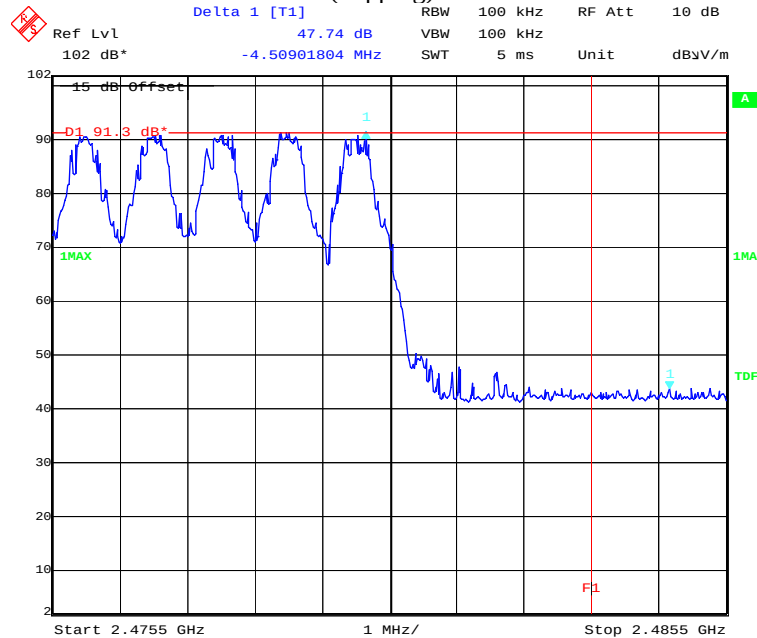
Plot 3: Marker-Delta Method (hopping)
