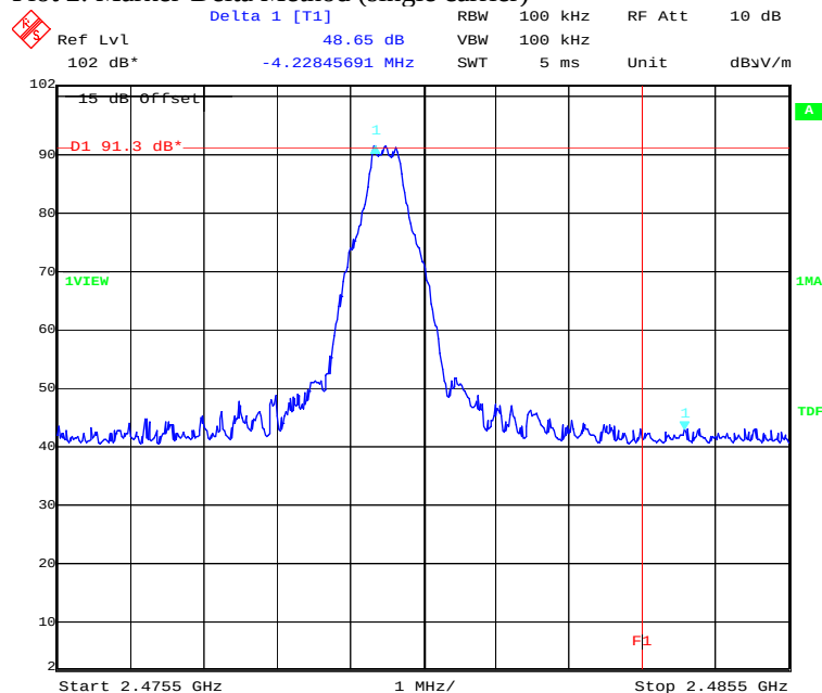
Plot 2: Marker-Delta Method (single carrier)
