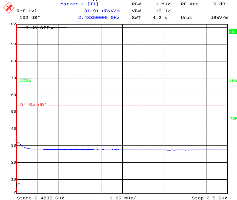
Plot 5: Restricted Bands high
