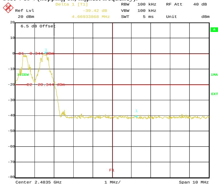
Plot 4 of 4 (hopping on, highest frequency):
