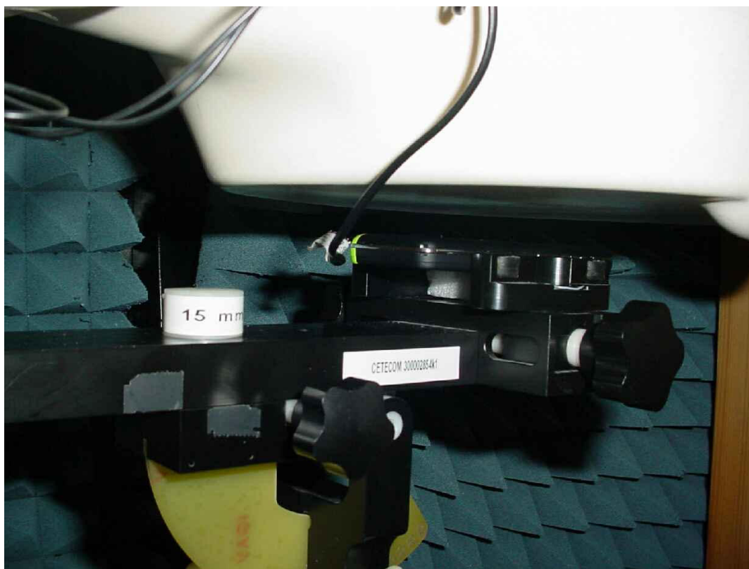
Photo 22: Test position body worn rear side (15 mm distance)
