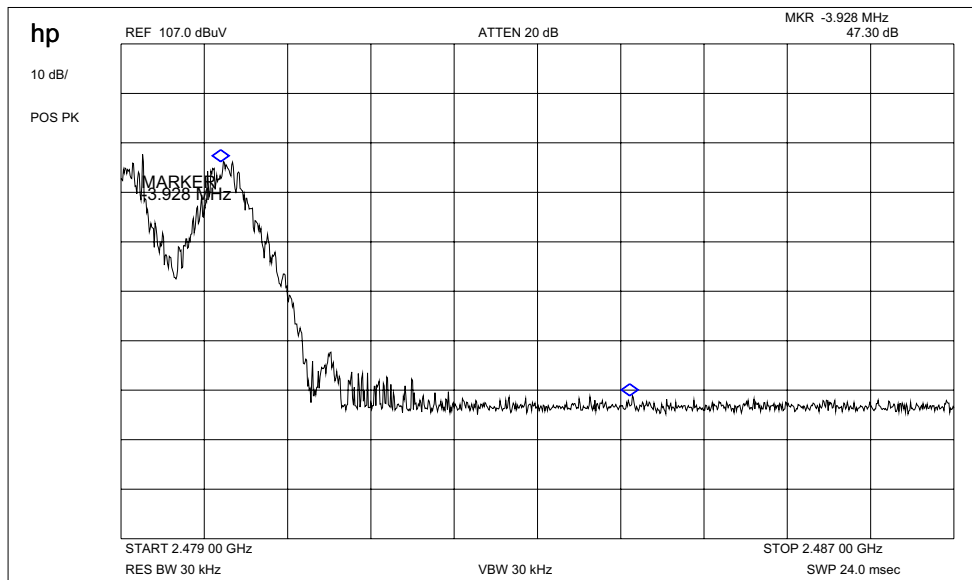
Plot 3: Marker-Delta Method (hopping)
