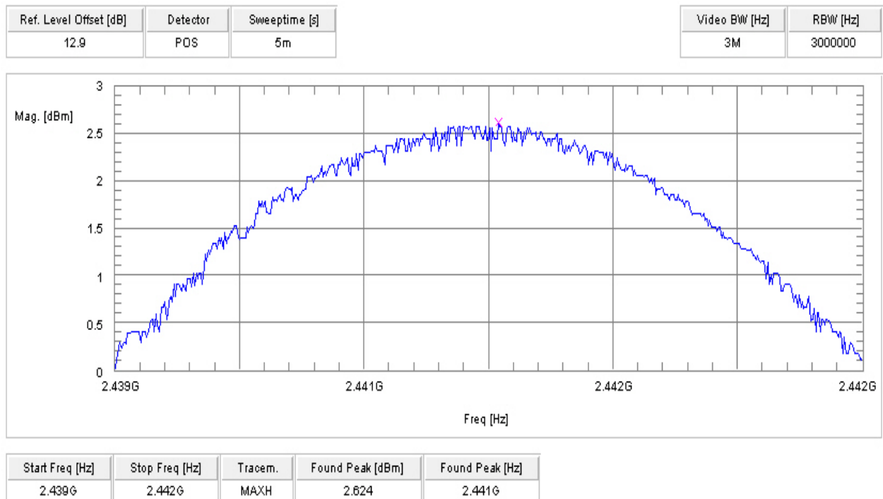
Plot 8 8DPSK
