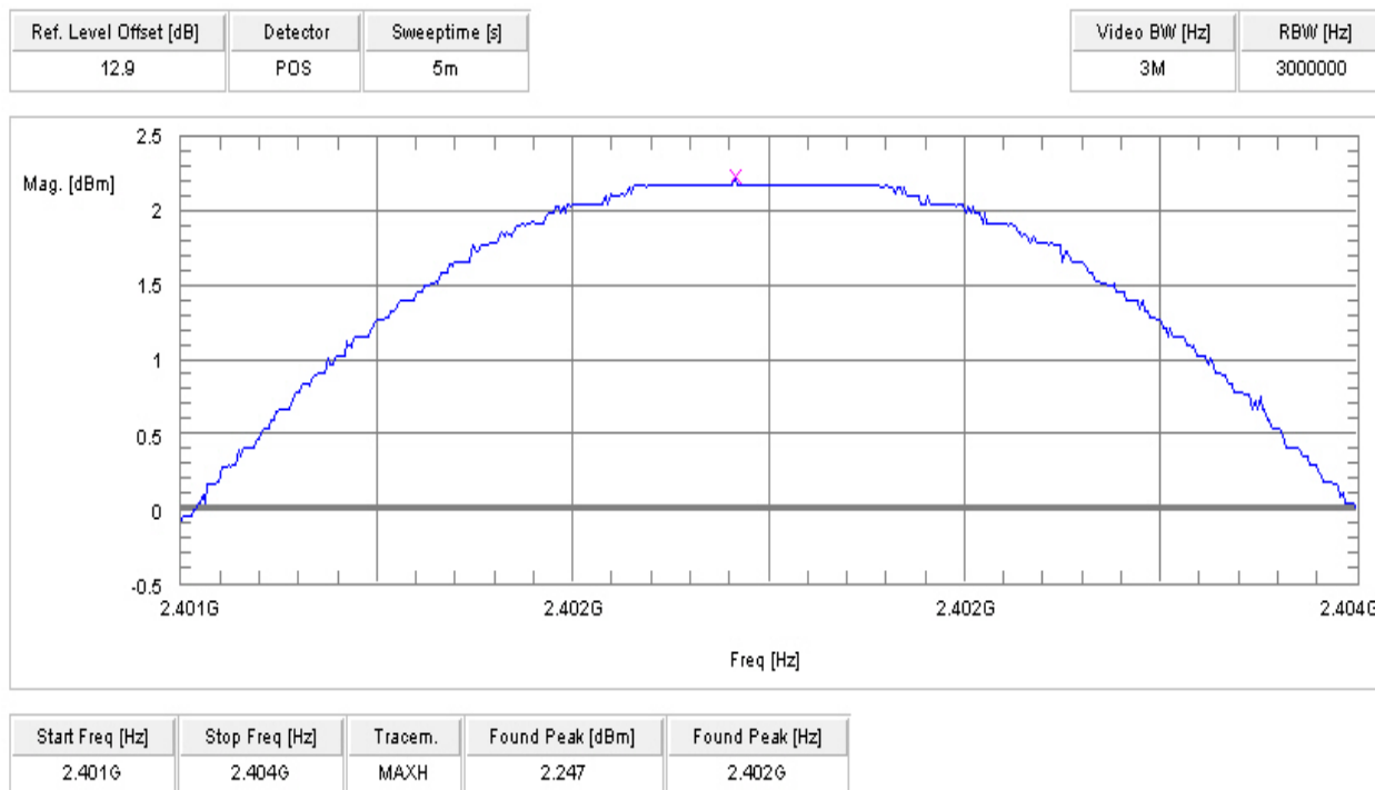
Plot 1 GFSK
