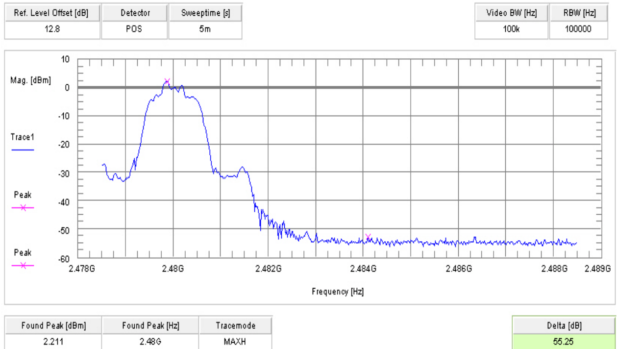
Plot 3 of 4 (hopping off, highest frequency):
