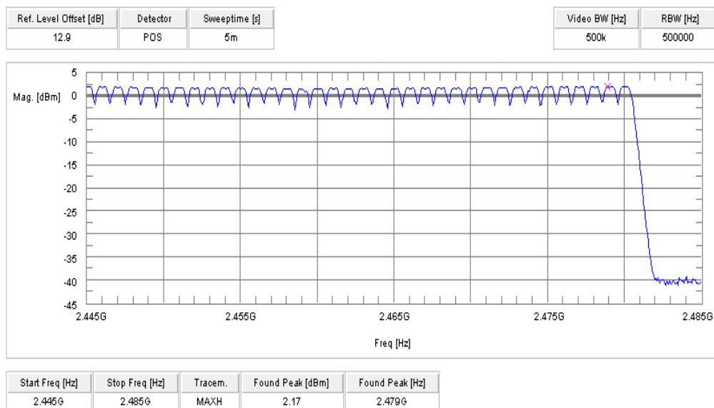
Plot 2 of 2:
