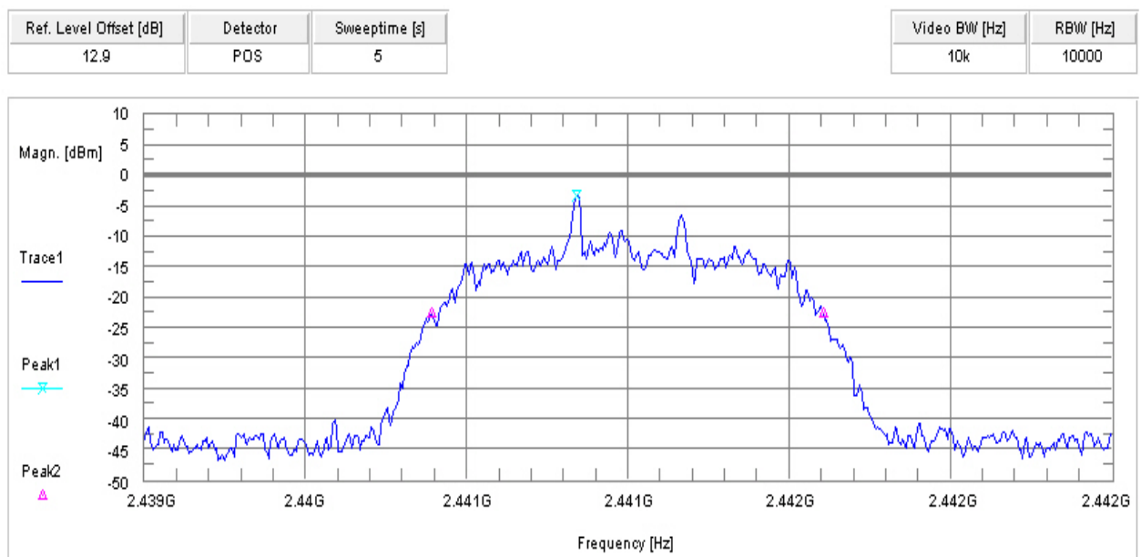
Plot 8 8DPSK
