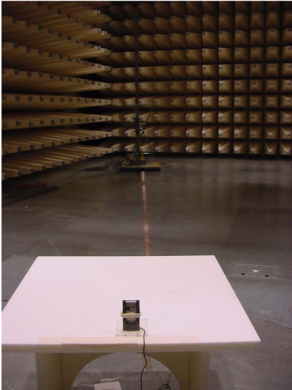
Photo 1: Radiated Emissions
