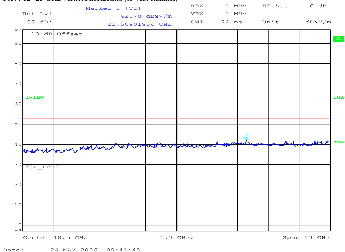
Plot : 12- 25 GHz vertical/horizontal (lowest channel)
