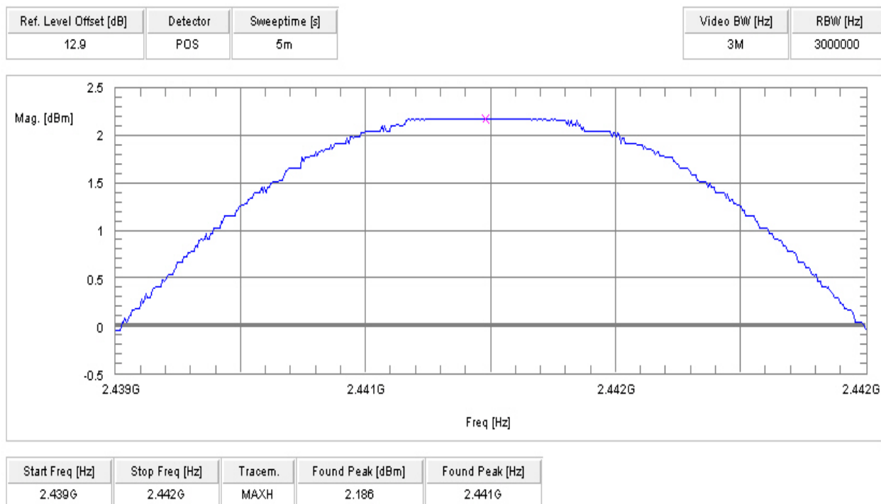
Plot 2 GFSK
