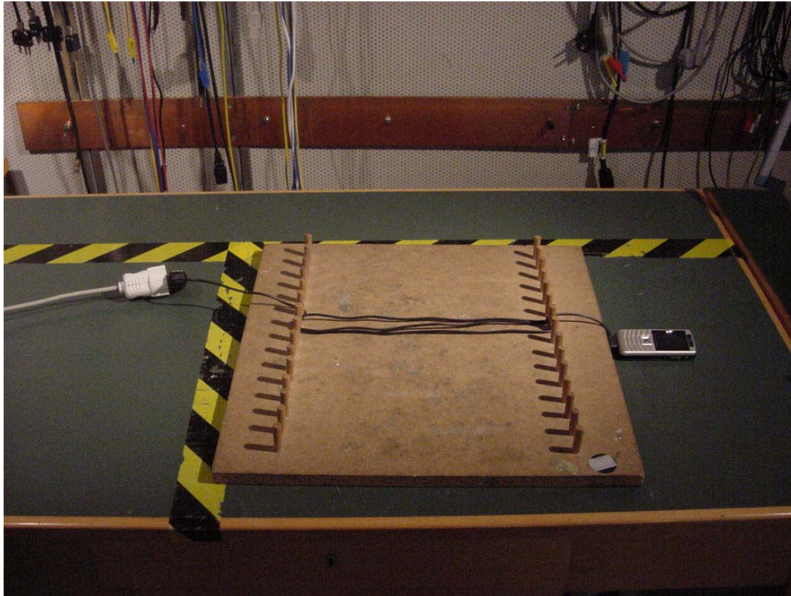
Photo 2: Conducted Emissions
