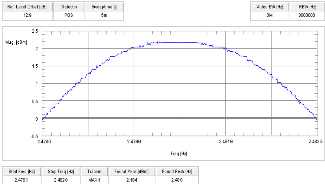
Plot 3 GFSK
