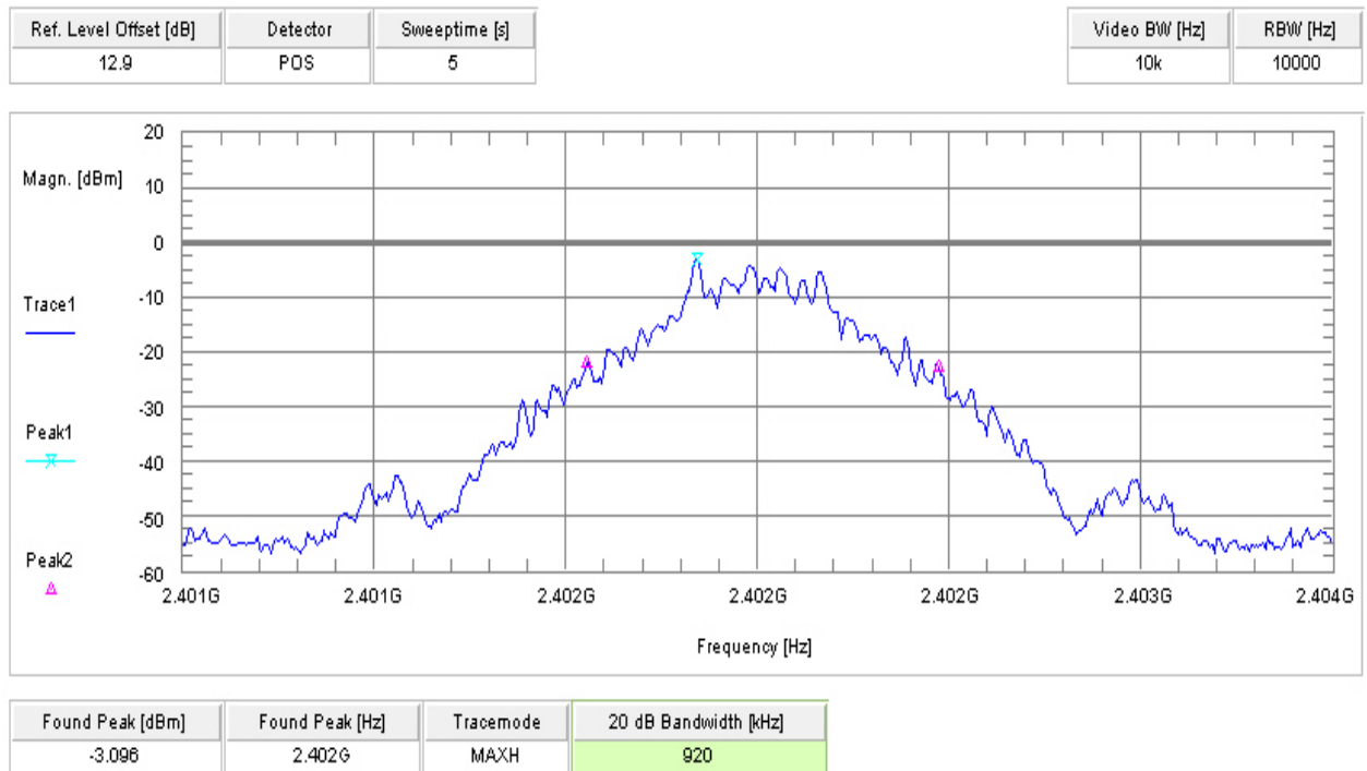
Plot 1 GFSK
