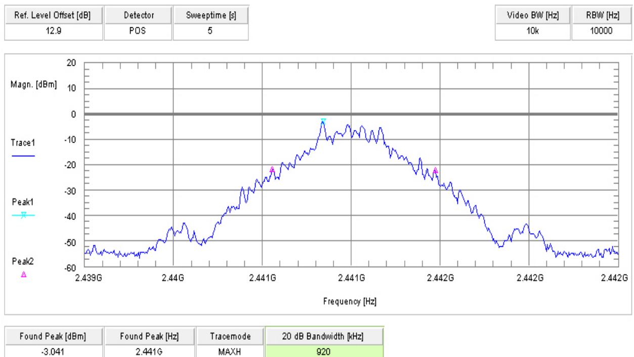
Plot 2 GFSK
