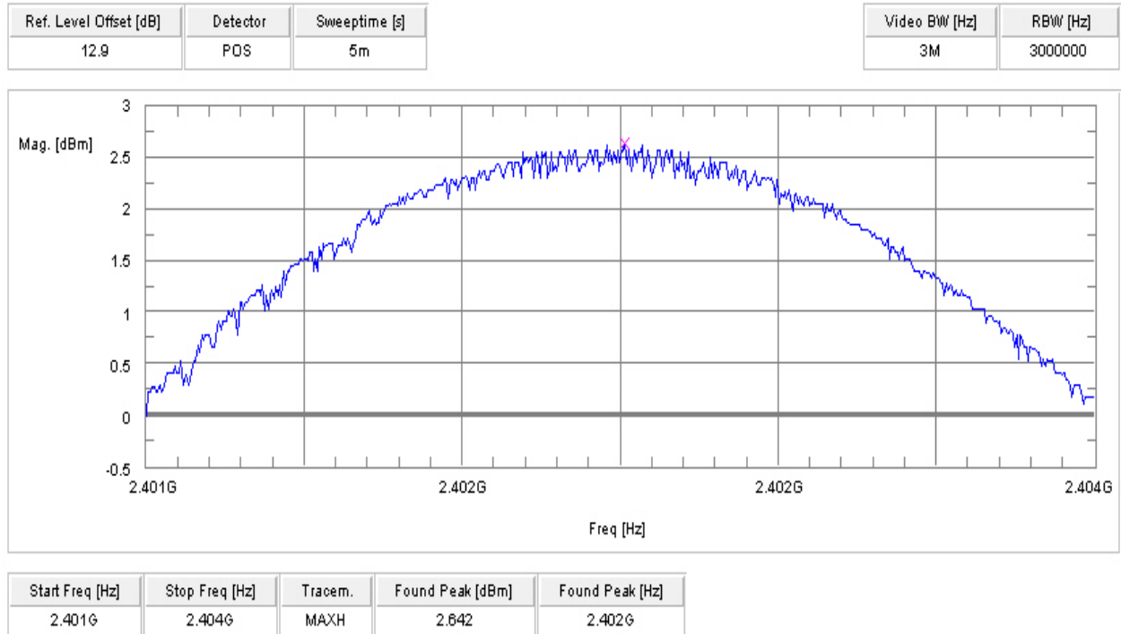
Plot 7 8DPSK
