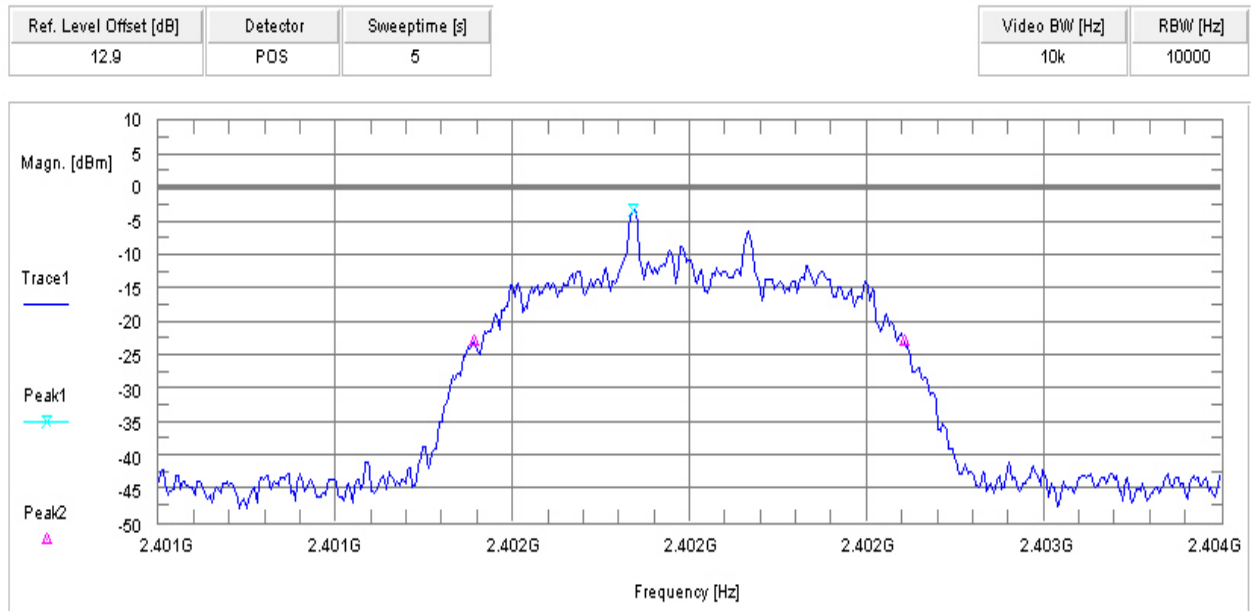
Plot 7 8DPSK
