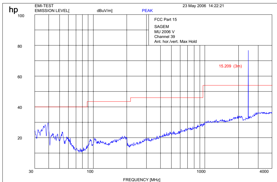
Plot : 0.03 - 4 GHz vertical/horizontal (middle channel)
