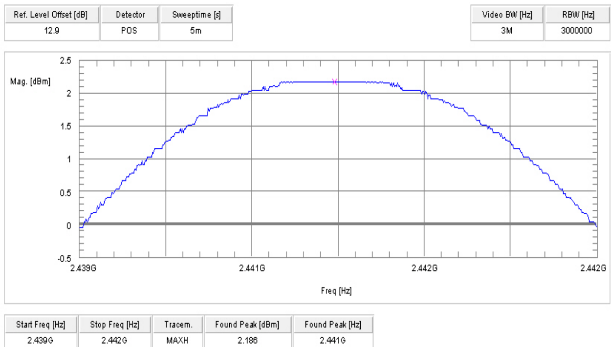
Plot 2 GFSK
