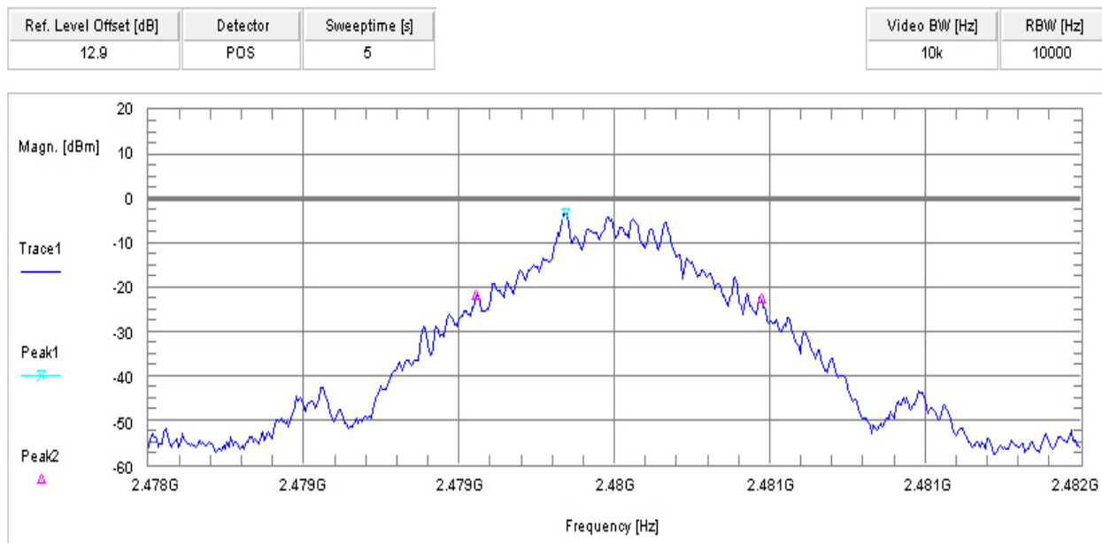
Plot 3 GFSK
