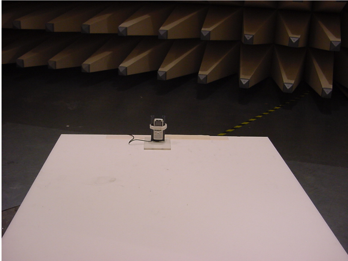
Photo 2: Radiated Emissions
