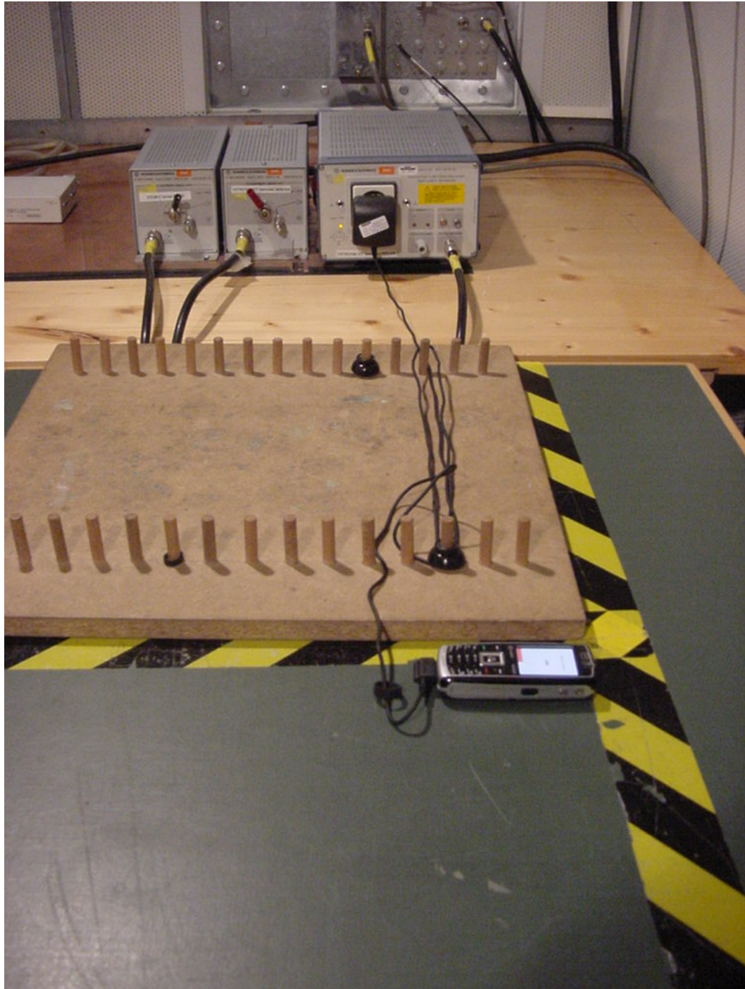
Photo 3: Conducted Emissions
