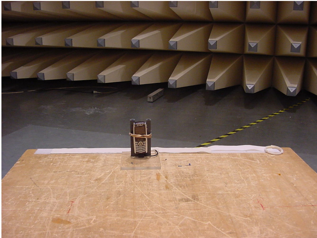
Photo 5 (Radiated Emissions):
