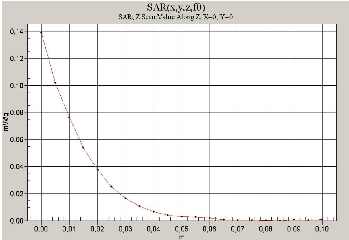
Z-axis scans 1900MHz head
