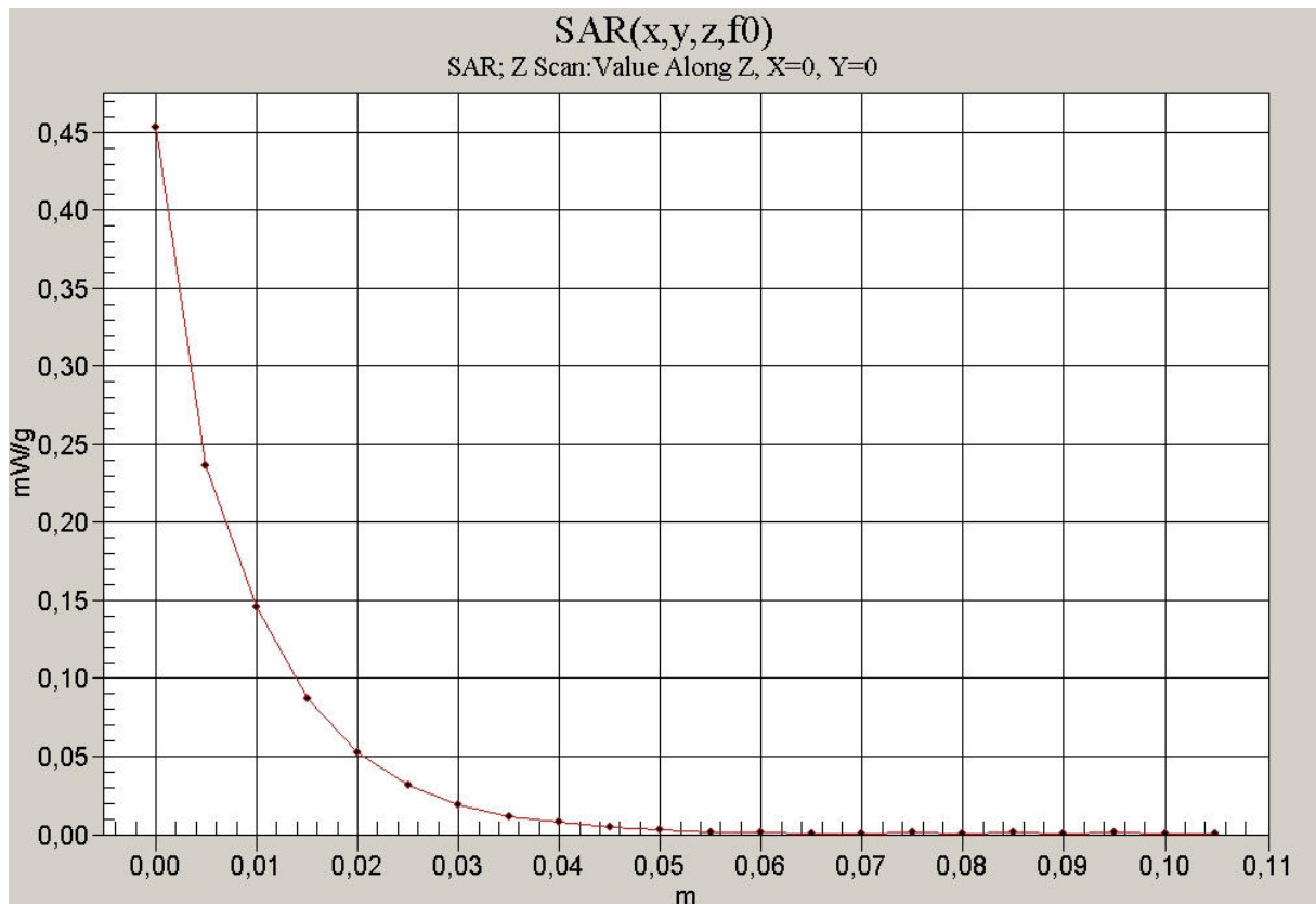
Z-axis scans 1900MHz body
