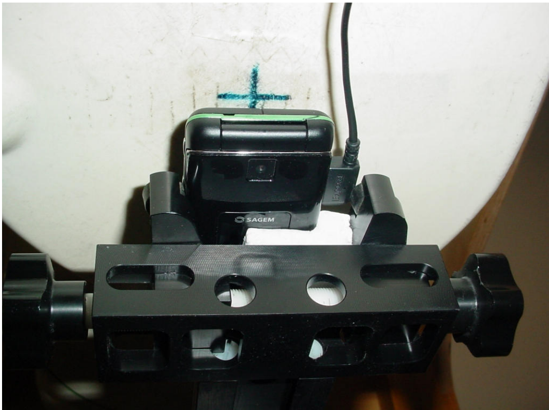
Photo 24: Test position body worn rear side (15 mm distance)
