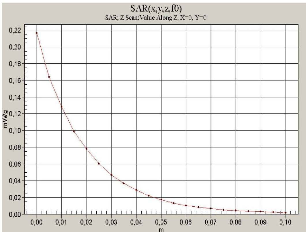
Photo 35: Z-scans 1900 MHz head
