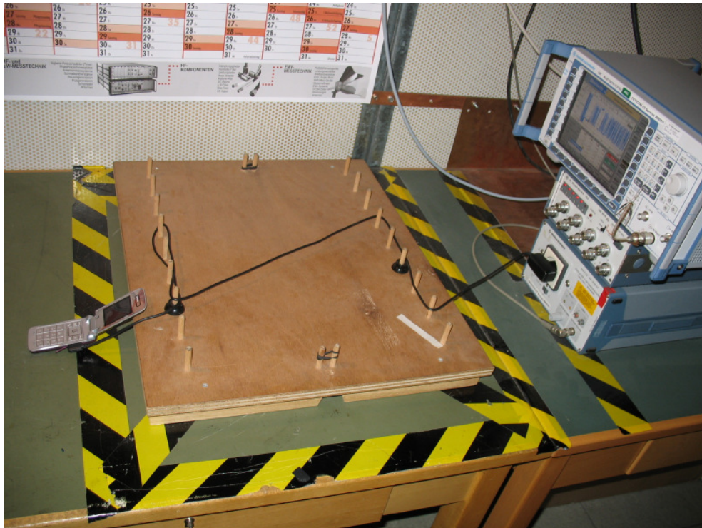
Photo 3: Conducted Test Set-up
