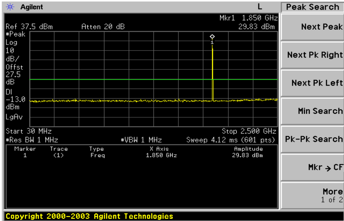
Figure 8-1: Out of Band emission at antenna terminals– PCS Channel Lowest
