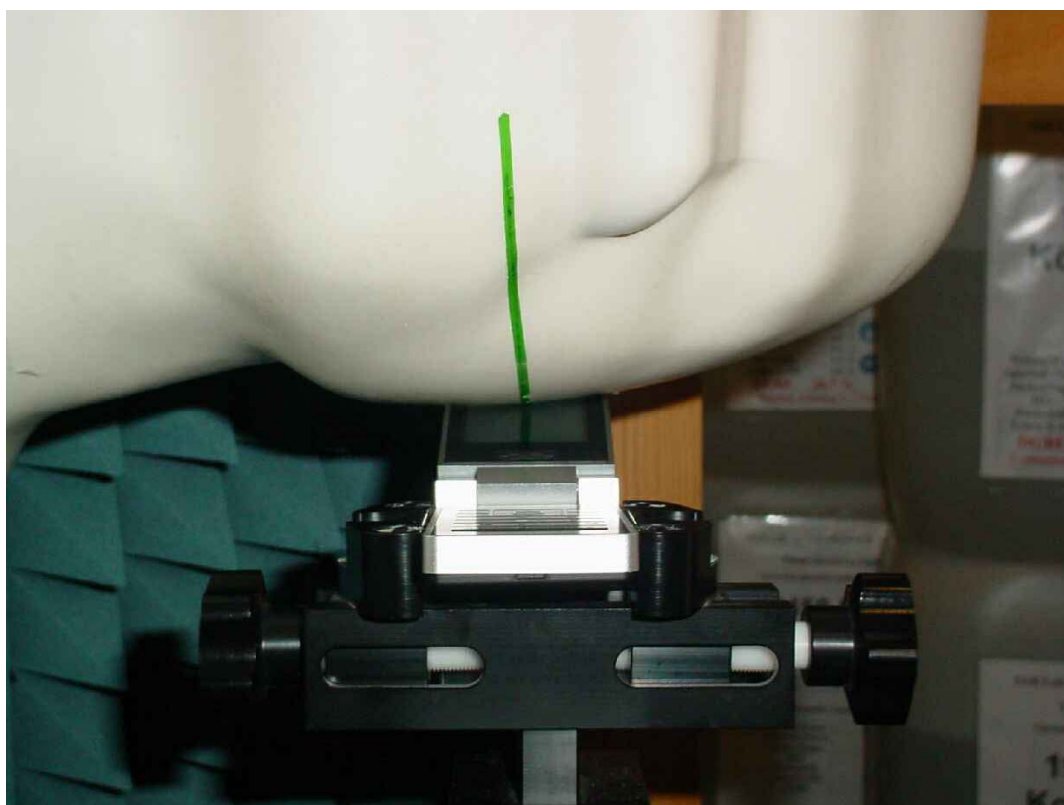
Photo 18: Test position left hand tilted 15°
