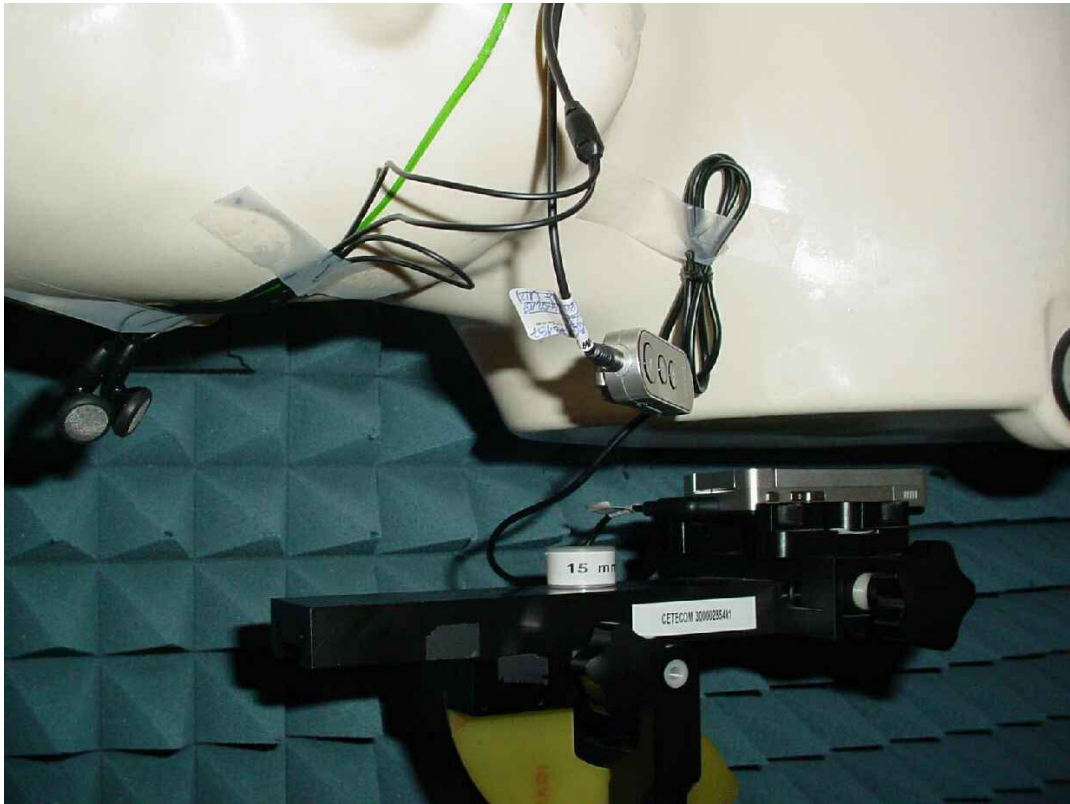
Photo 26: Test position body worn front side (distance 15 mm)
