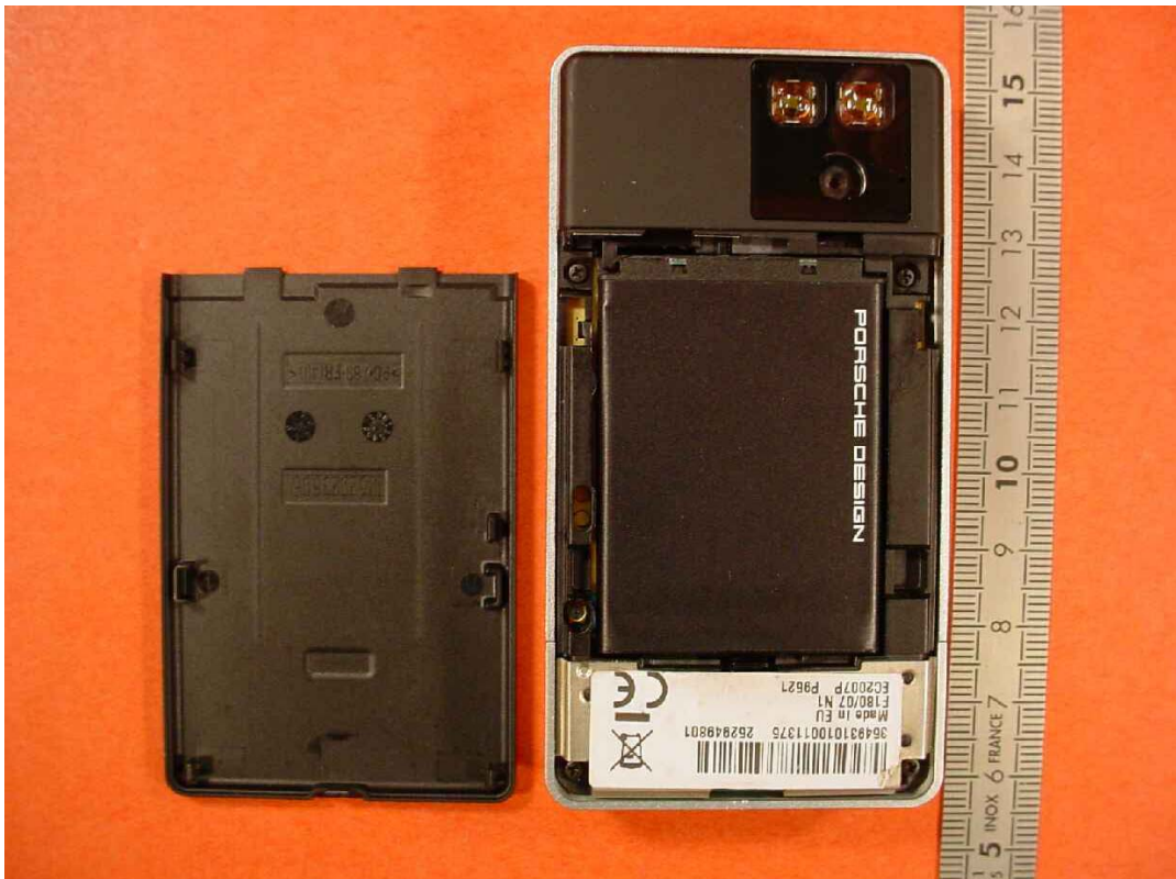
Photo 12: DUT - rear over view (open)
