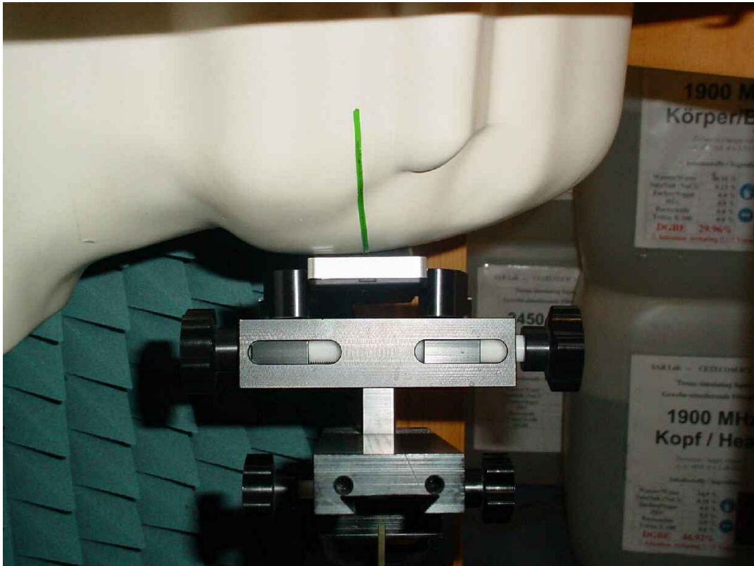
Photo 16: Test position left hand touched
