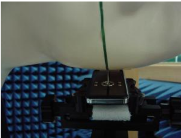
Fig.5 Photograph of the Left Hand Side Tilt status
