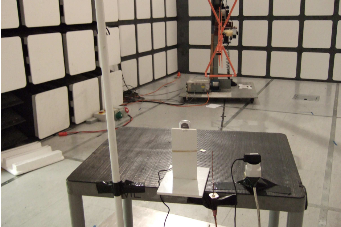
Sagem DC2006a – Test Set Up Photo 1 (Radiated Emissions)
