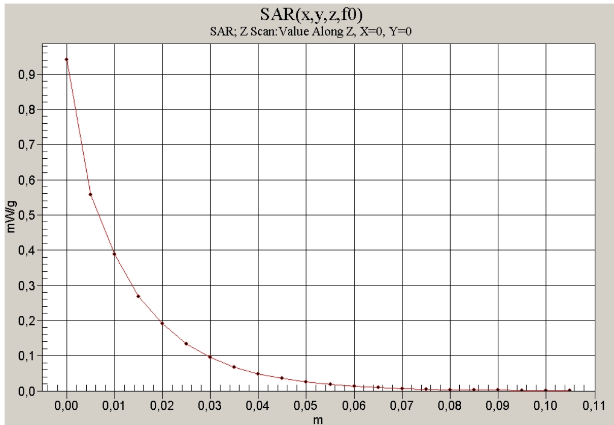
850 MHz head
