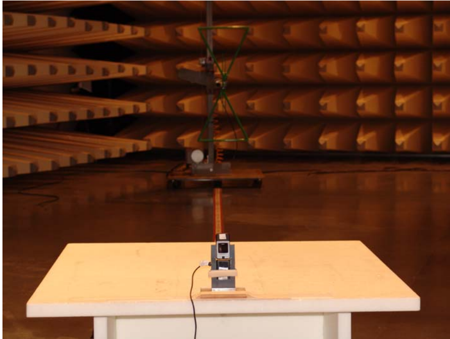
Photo 2: Radiated Emissions
