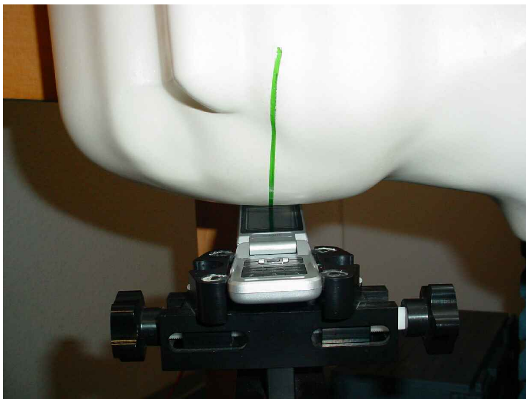
Photo 21: Test position right hand tilted 15°
