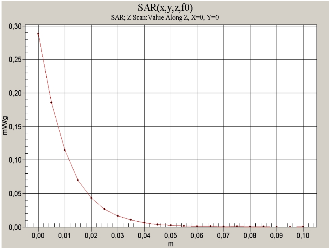
Photo 37: Z-axis scans 1900 MHz body
