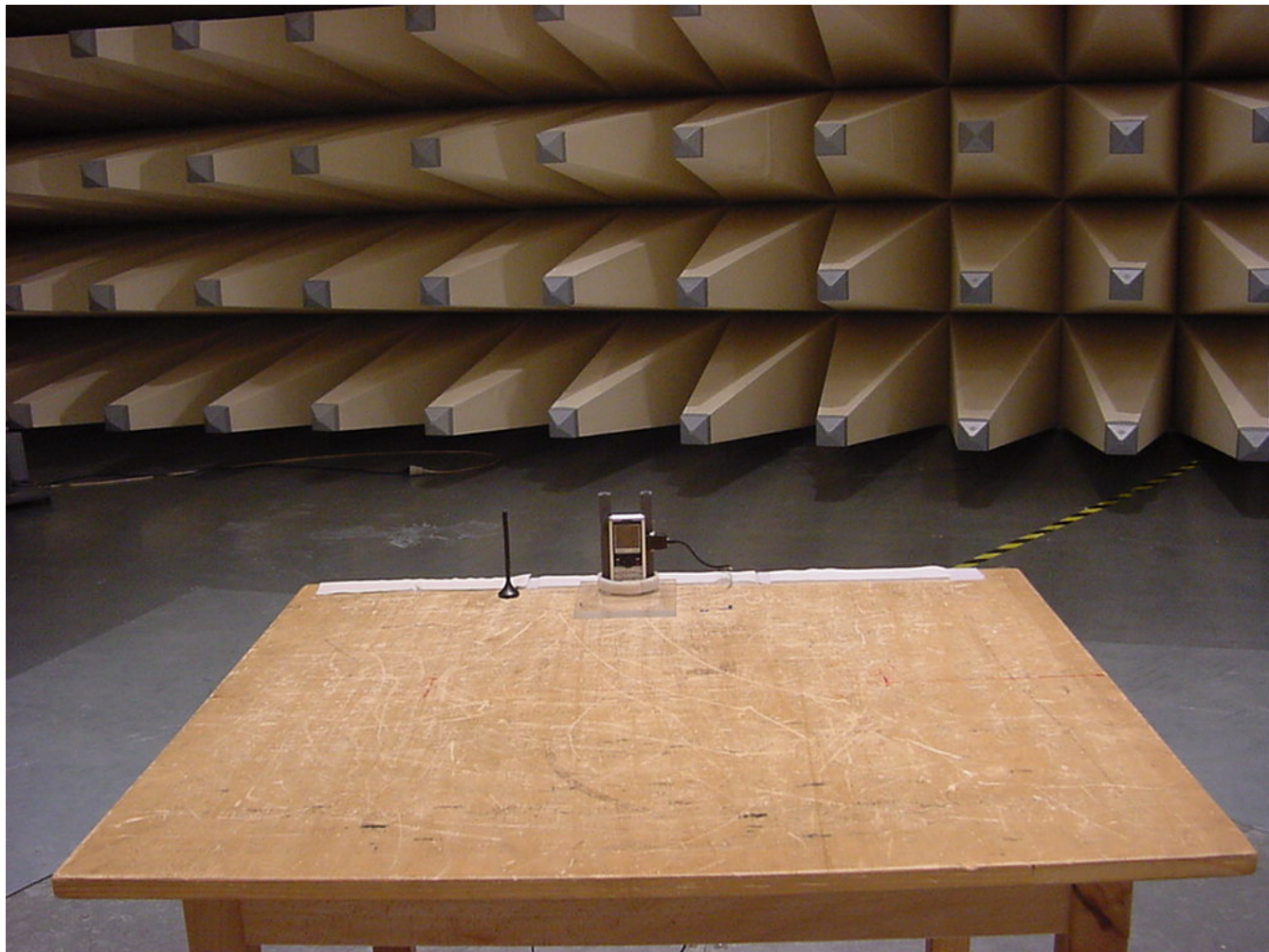
Photo 3 (Radiated Emissions):
