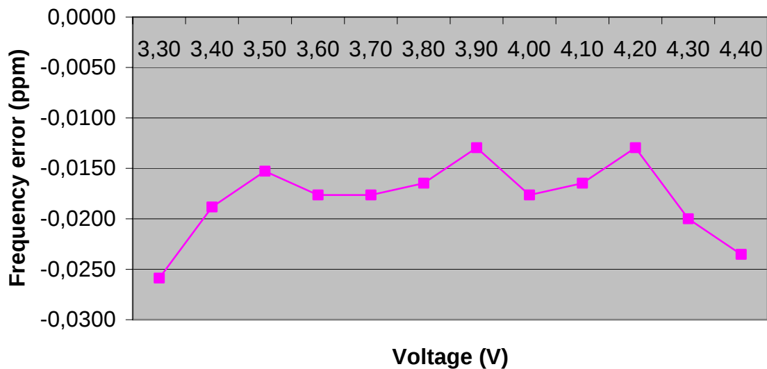
Frequency Error vs. Voltage
