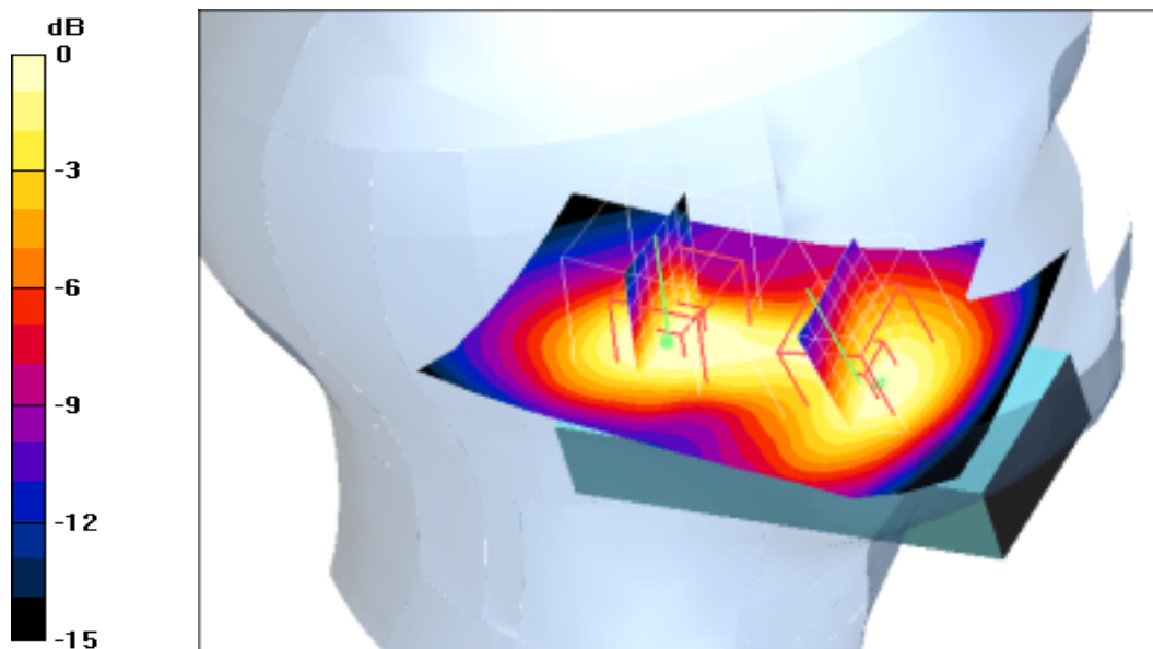
0 dB = 0.352mW/g
