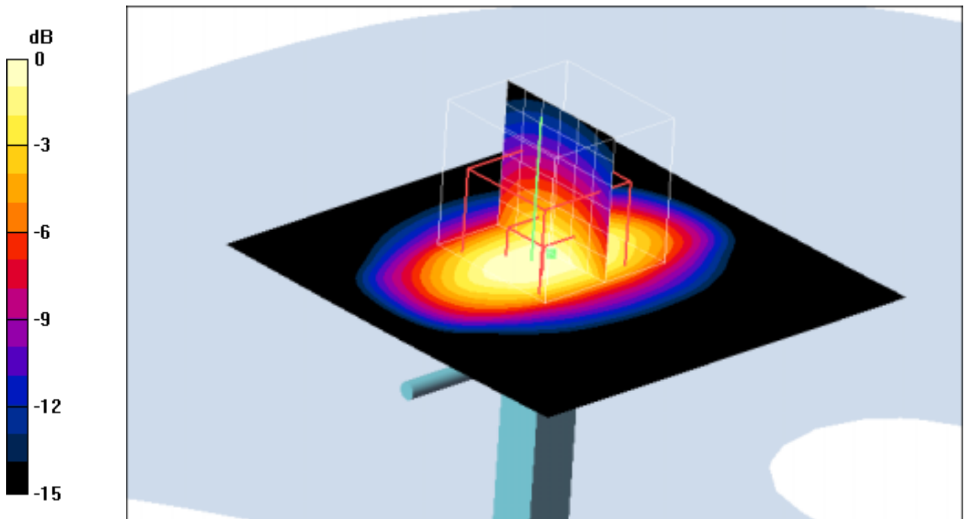
0 dB = 46.7mW/g
