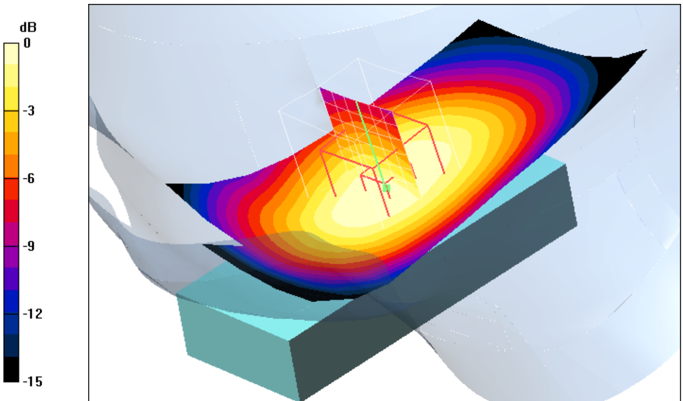
0 dB = 0.557mW/g
