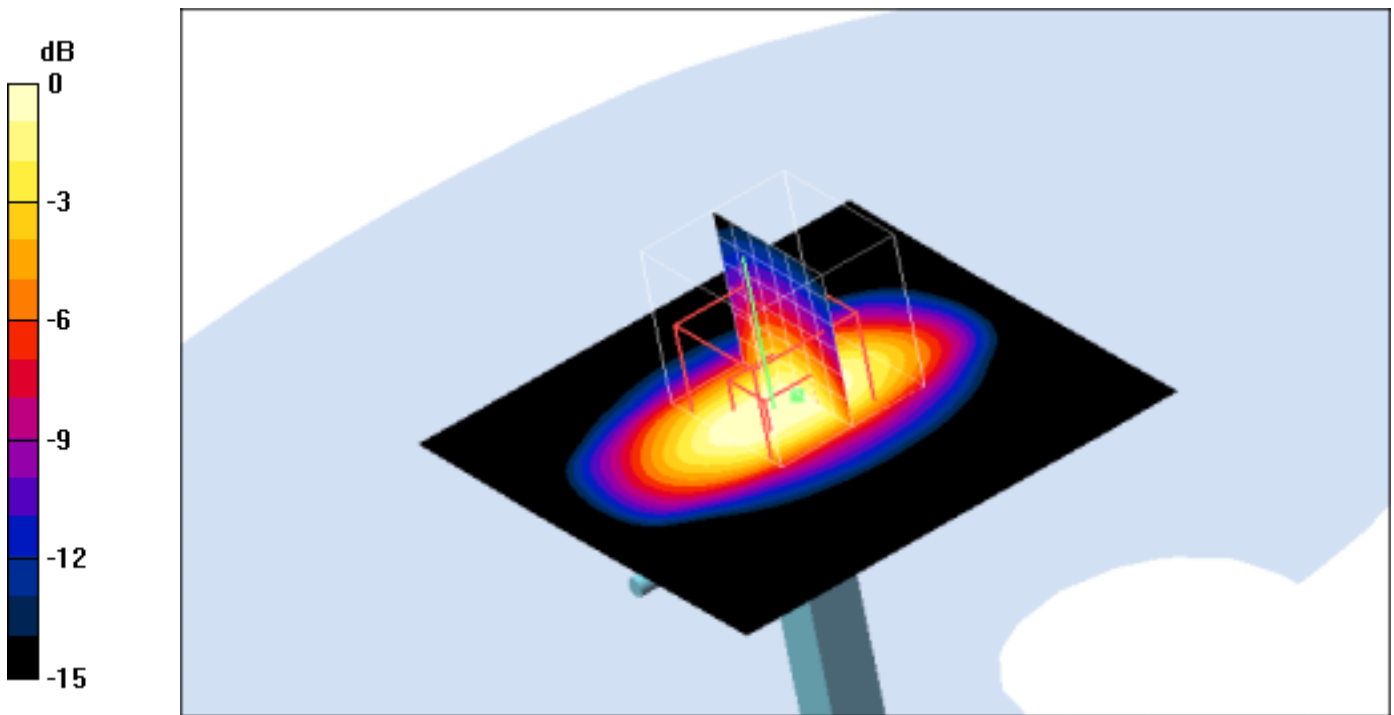
0 dB = 47.5mW/g
