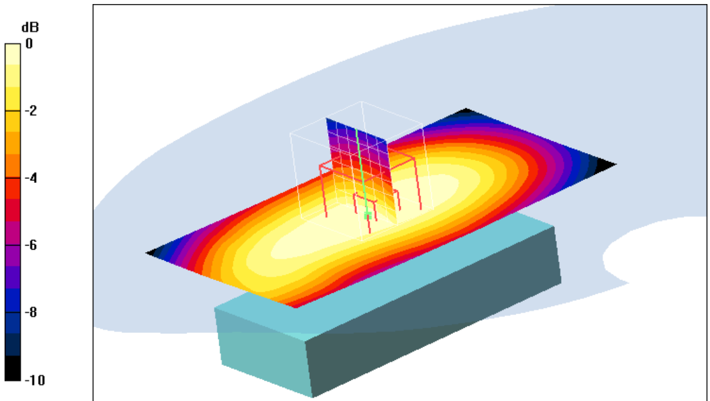
0 dB = 0.112mW/g
