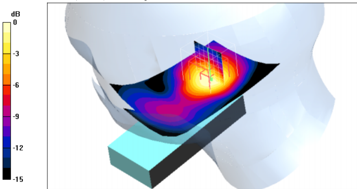
0 dB = 0.368mW/g
