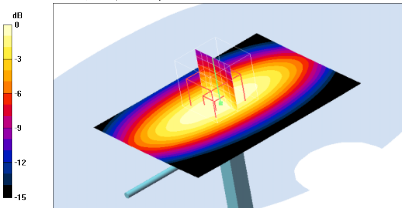
0 dB = 11.6mW/g
