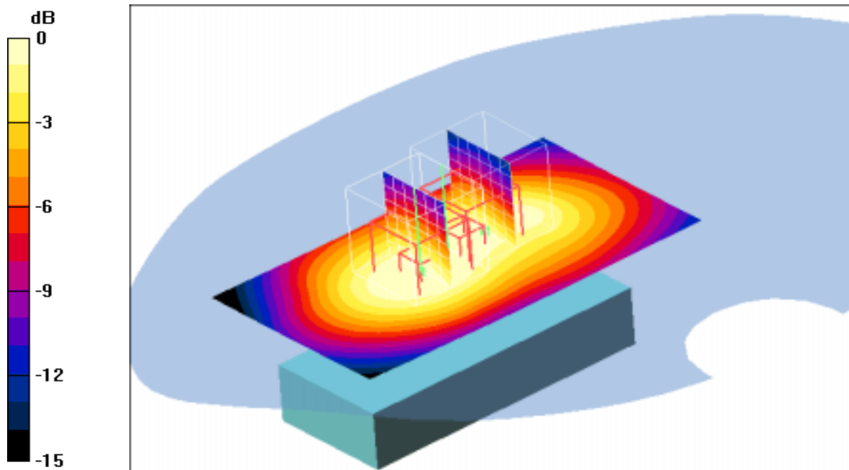
0 dB = 0.247mW/g
