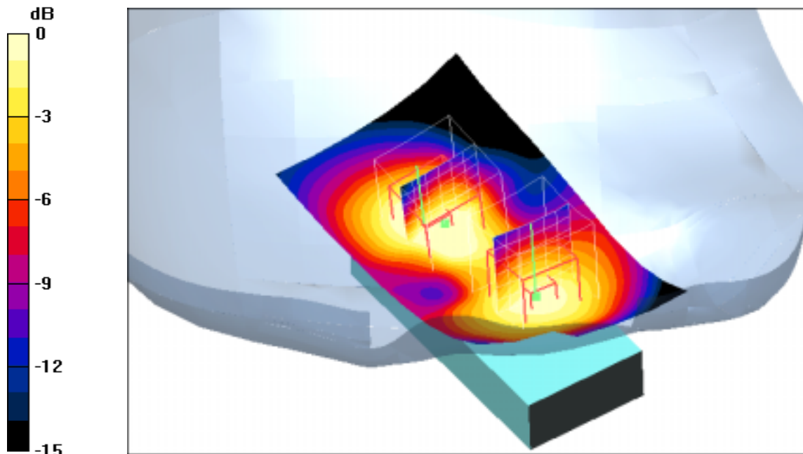
0 dB = 0.330mW/g
