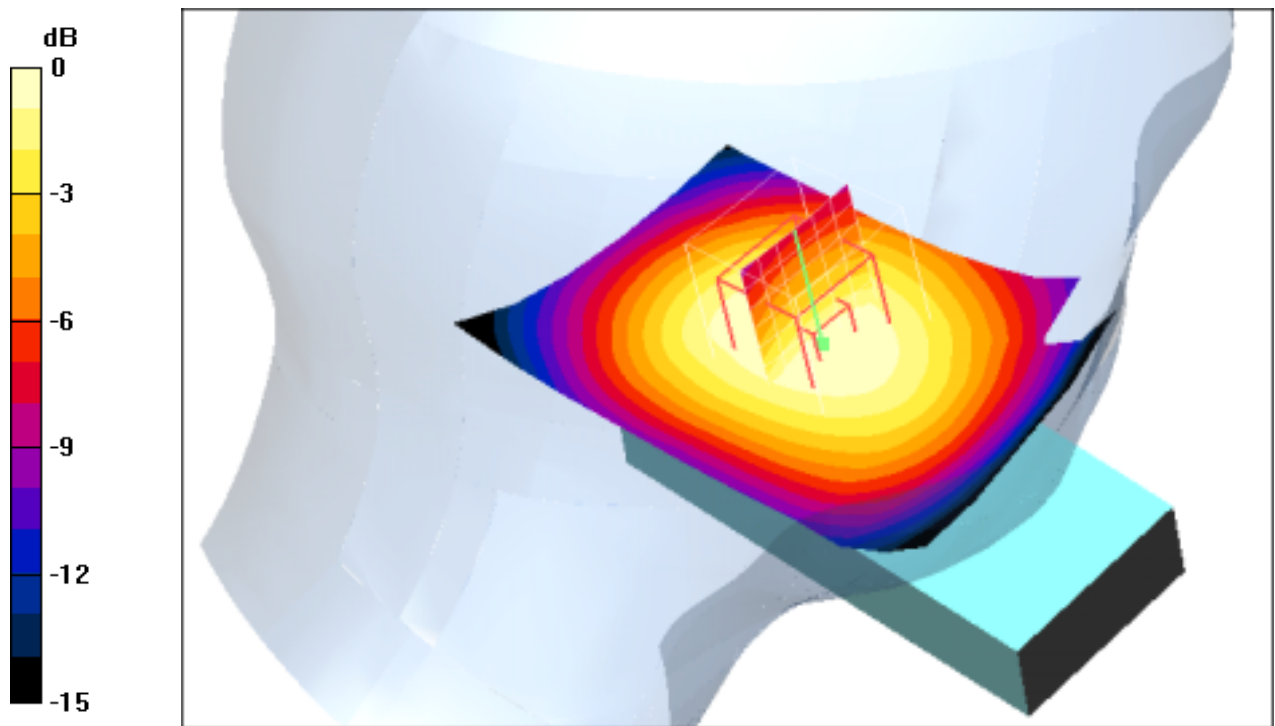
0 dB = 0.344mW/g
