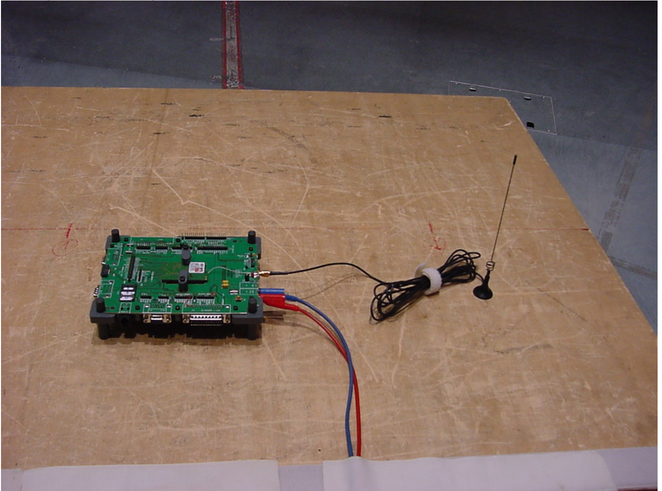
Photo 2 (Radiated Emissions):
