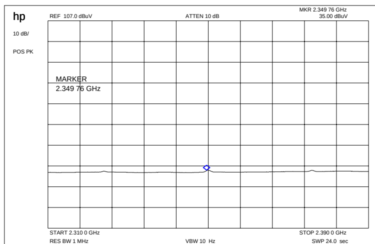
Plot 4: Restricted Bands low
