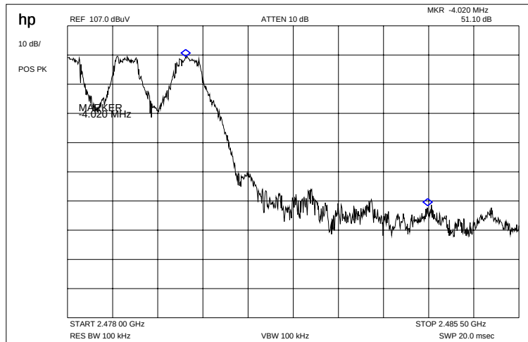
Plot 3: Marker-Delta Method (hopping)
