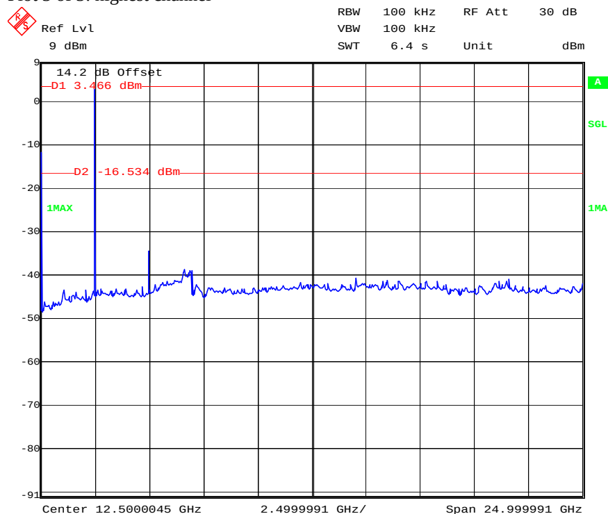
Plot 3 of 3: highest channel
