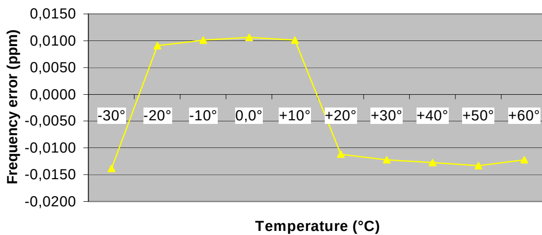
FREQUENCY ERROR VERSUS TEMPERATURE
