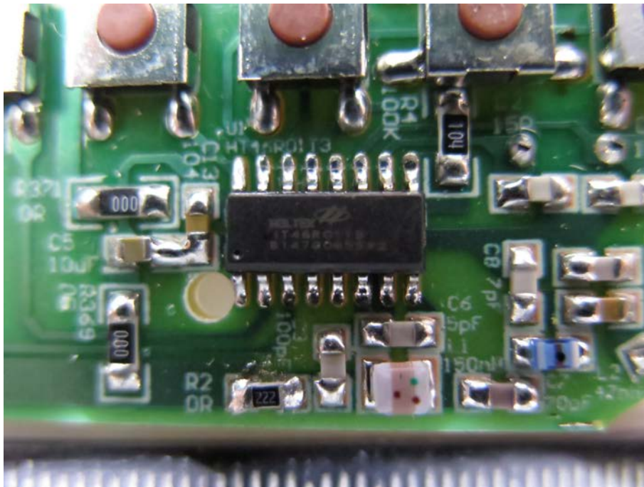
View of the Chip IC: HT46R01T3
