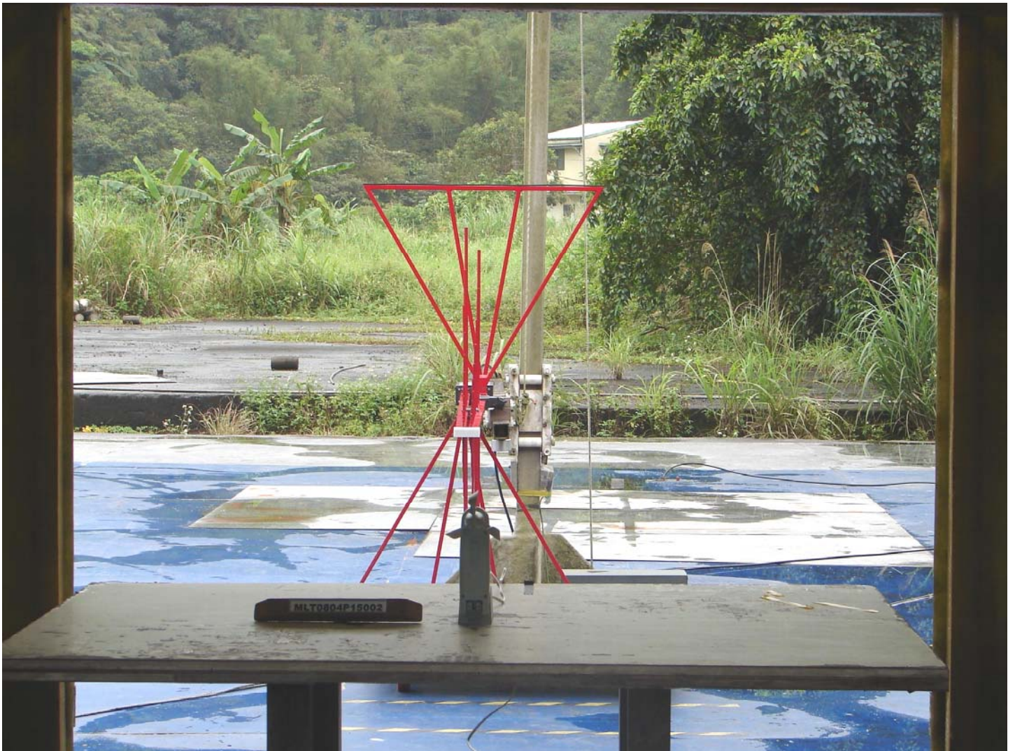
Front View of The Test Configuration
