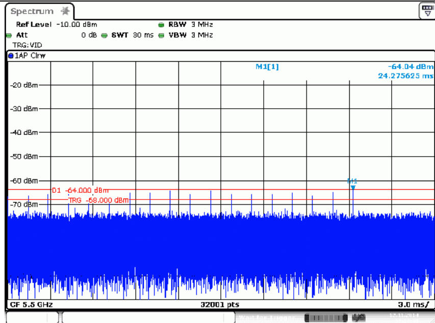
Radar test signal type 1 / 5500MHz
