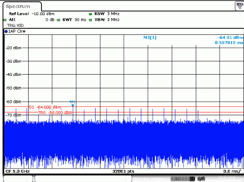
Radar test signal type 1 / 5300MHz
