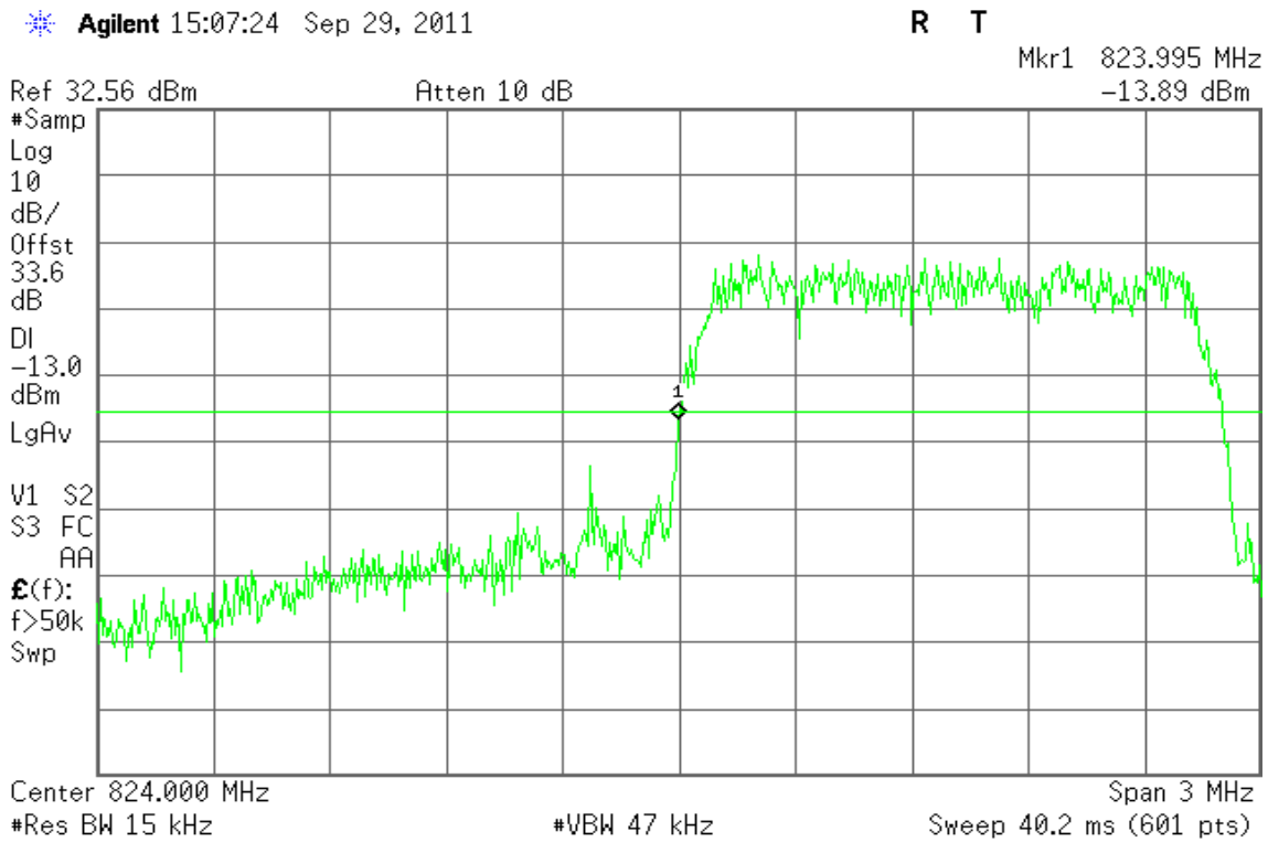
Figure 12-1: Band Edge emissions – CDMA2000 1xEVDO / CH Low
