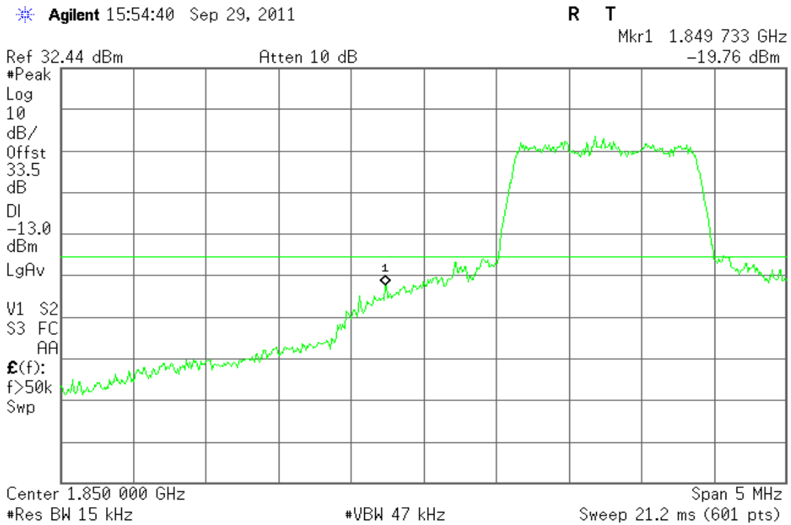
Figure 13-1: Band Edge emissions – CDMA2000 1xRTT / CH Low
