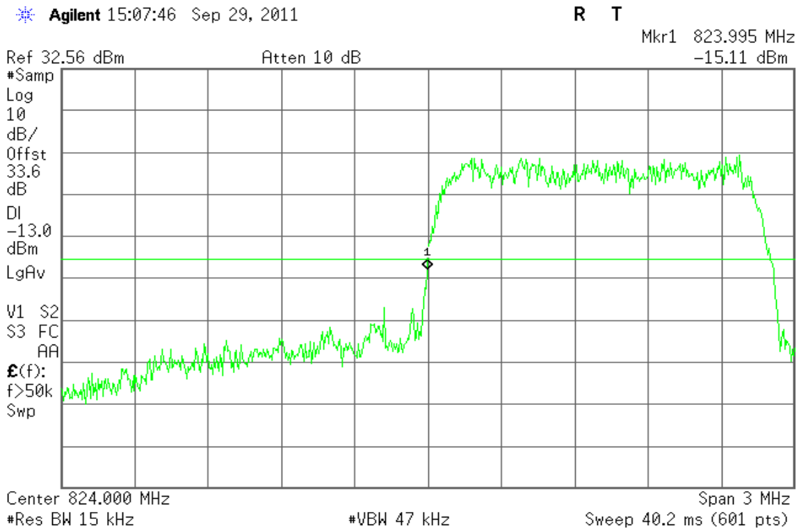
Figure 11-1: Band Edge emissions – CDMA2000 1xRTT / CH Low
