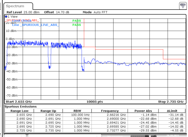
100RB#0+75RB#0_High Range
