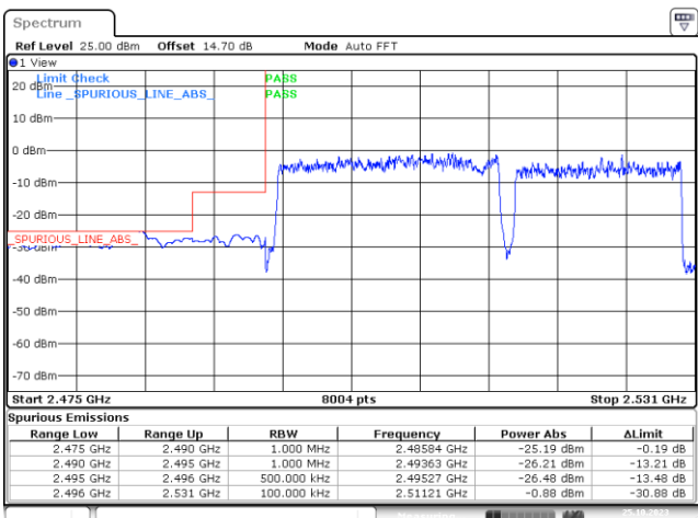
100RB#0+75RB#0_Low Range
