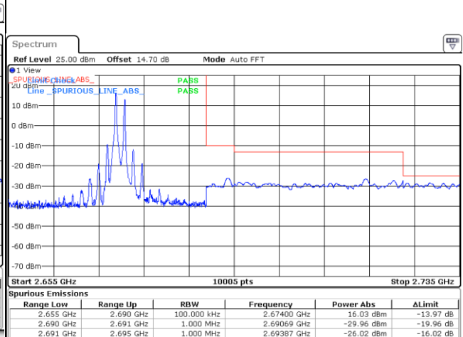
1RB#99+1RB#0_High Range
