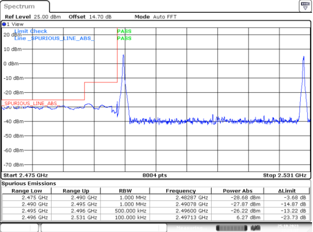
1RB#0+1RB#74_Low Range
