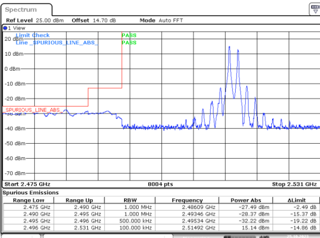
1RB#99+1RB#0_Low Range
