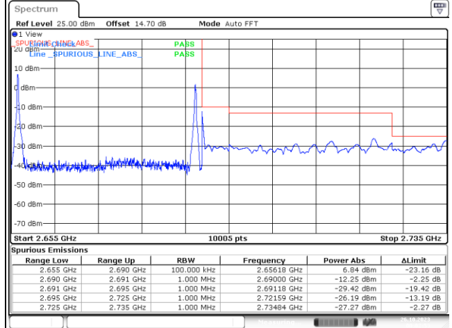
1RB#0+1RB#74_High Range
