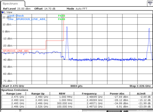
1RB#0+1RB#99_Low Range
