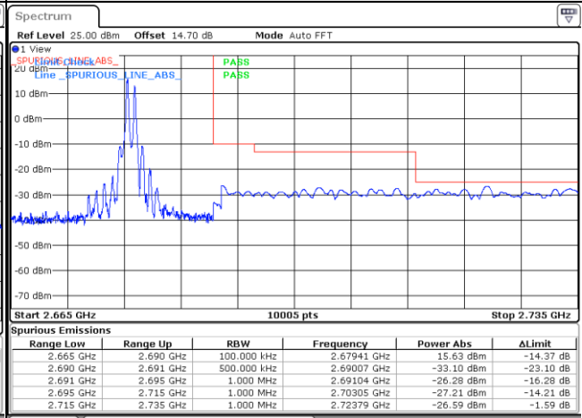
1RB#74+1RB#0_High Range
