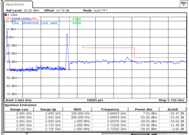
1RB#0+1RB#49_High Range
