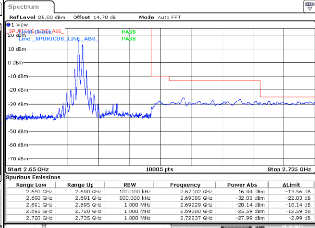
1RB#49+1RB#0_High Range
