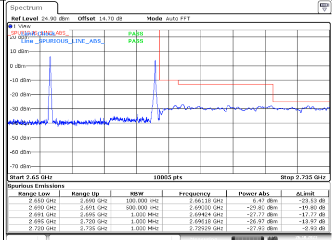
1RB#0+1RB#99_High Range
