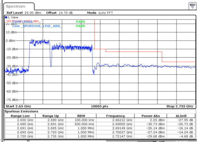
50RB#0+100RB#0_High Range
