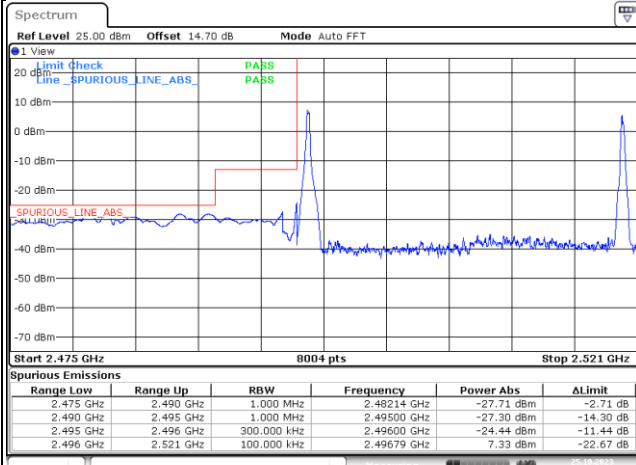
1RB#0+1RB#49_Low Range
