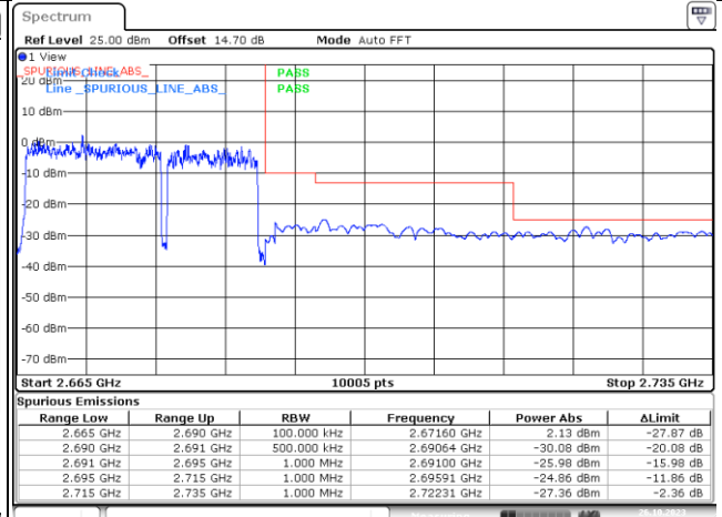
75RB#0+50RB#0_High Range
