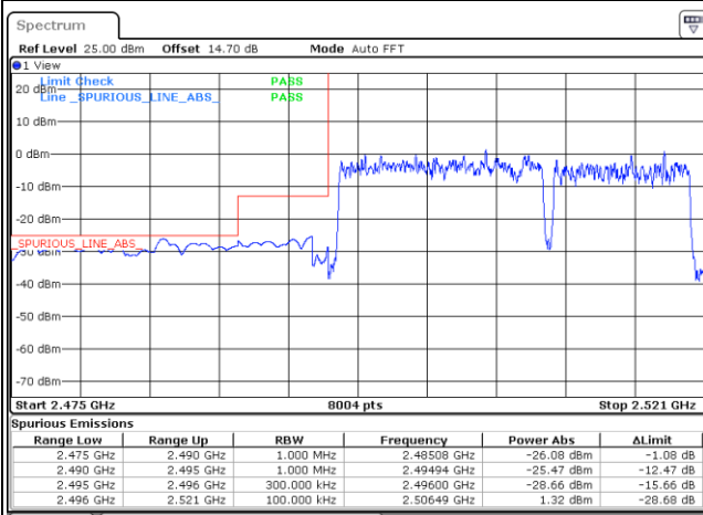
75RB#0+50RB#0_Low Range
