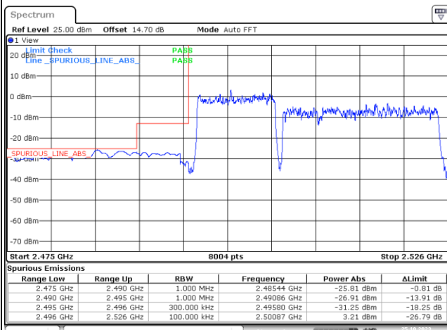
50RB#0+100RB#0_Low Range
