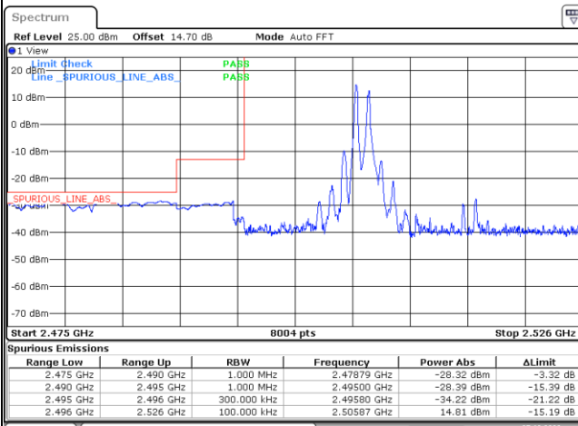
1RB#49+1RB#0_Low Range
