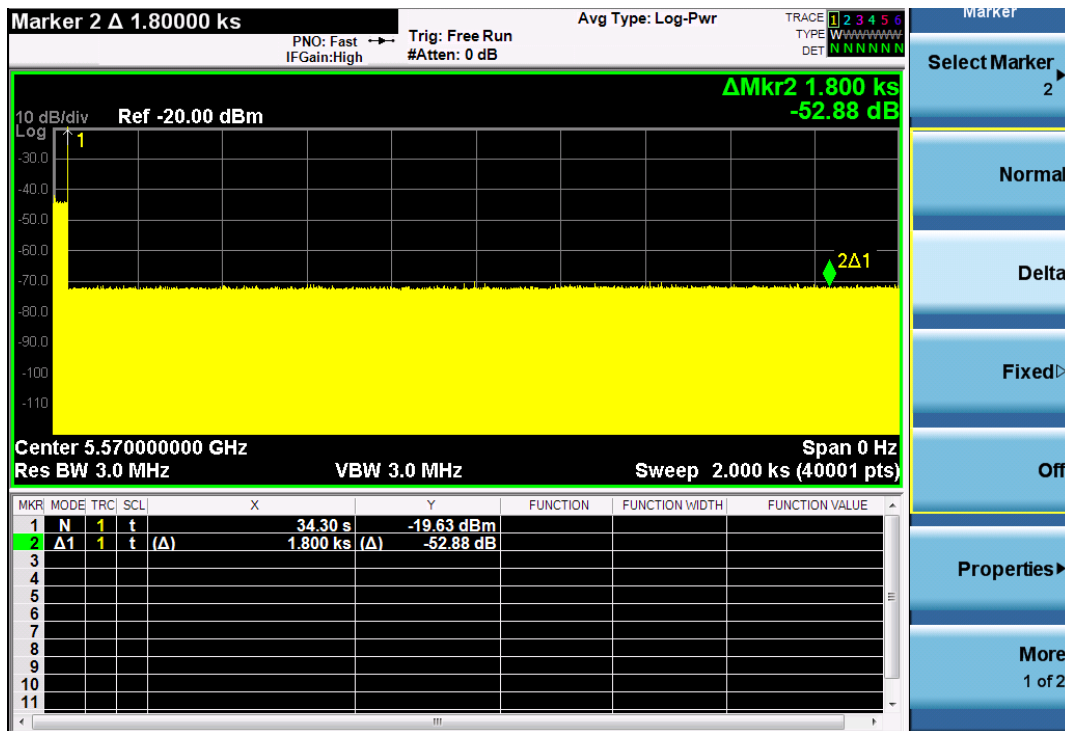
Test Bandwidth / Channel : 160MHz / 5570 MHz
