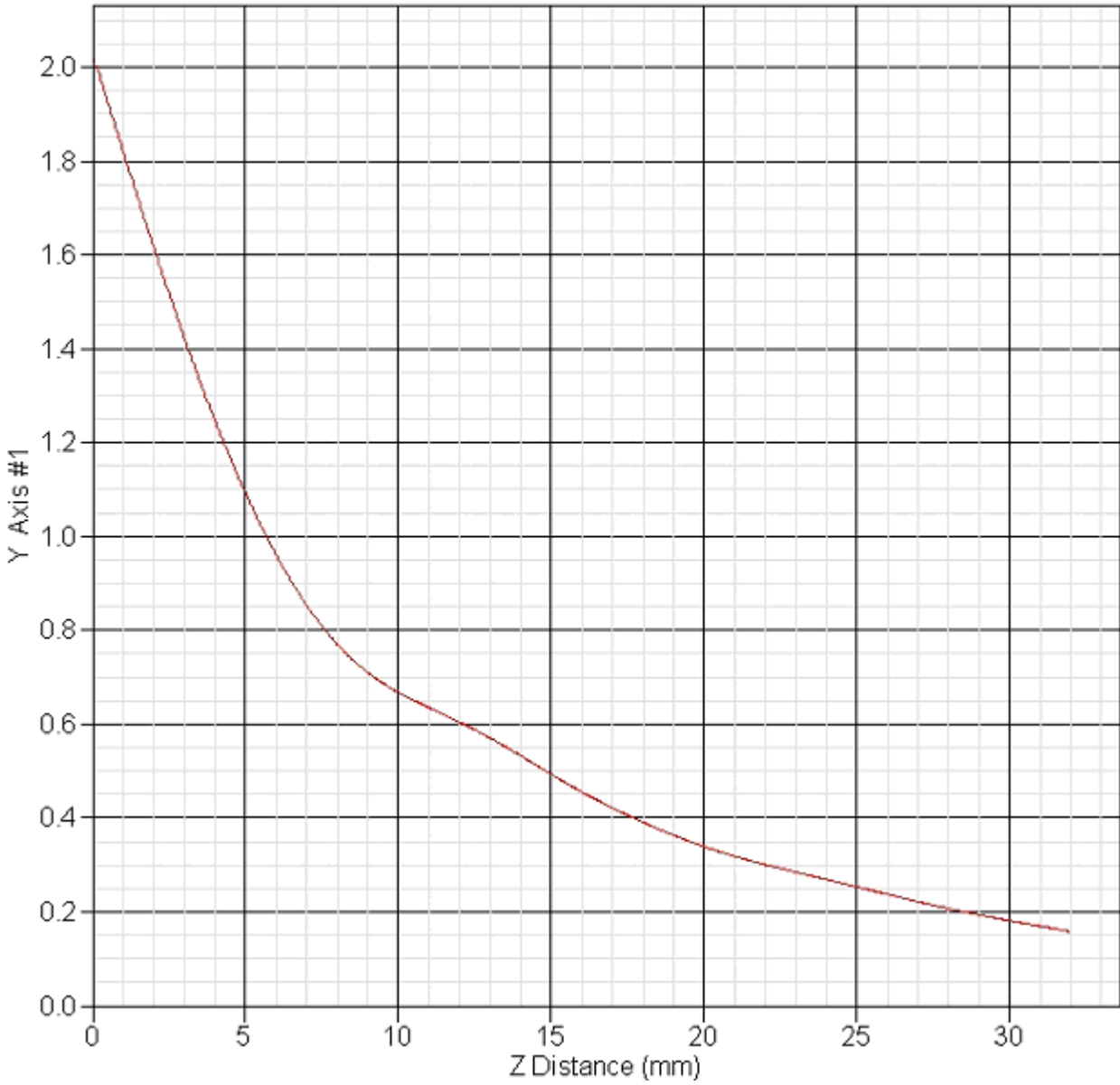
SAR-Z Axis at Hotspot x:70.20 y:-10.20
