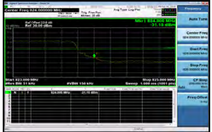
Part 90_Band26_10MHz_QPSK_1_0_LowCH26740
