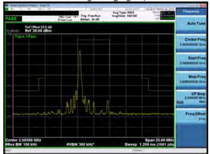
Band 41_16QAM_5M_RB1,24
