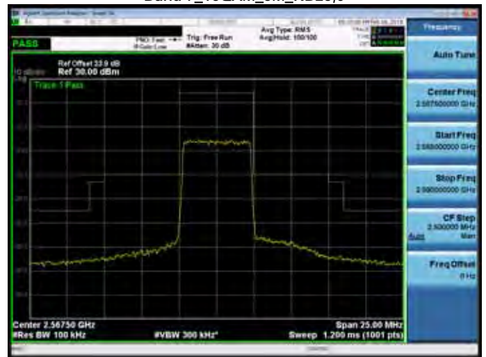
Band 7_16QAM_5M_RB25,0
