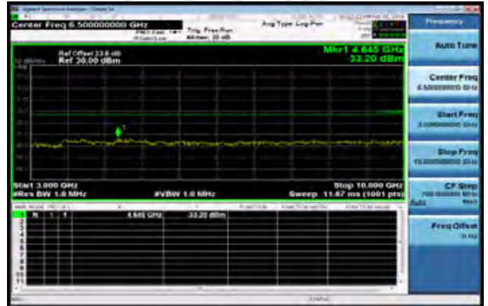
3GHz-10GHz_Band13_5MHz_QPSK_1_0_MidCH23230-782
