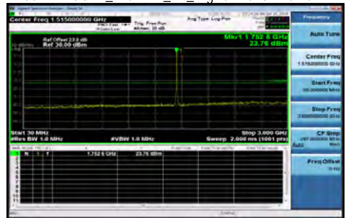
30MHz~3GHz_WCDMA_B4_HighCH1513-1752.6
