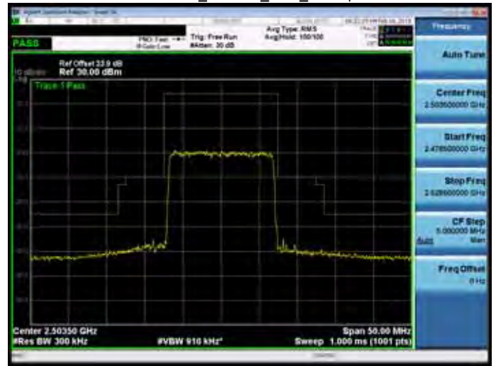
Band 41_16QAM_15M_RB1,0
