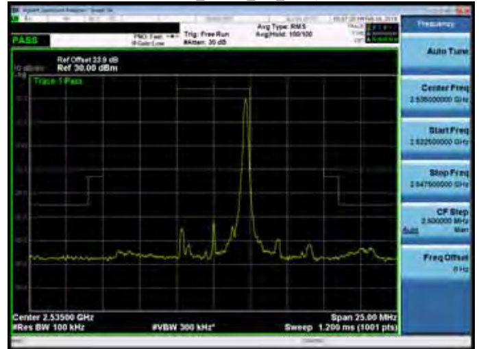
Band 7_QPSK_5M_RB25,0
