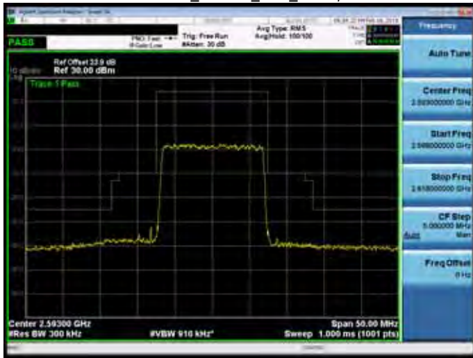
Band 41_16QAM_15M_RB1,0
