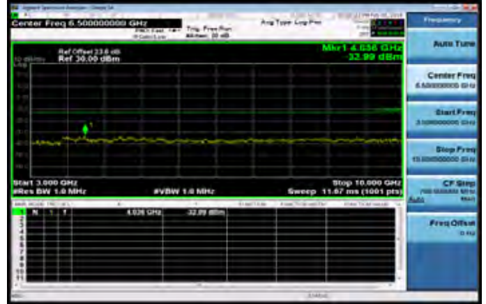
3GHz-10GHz_Band12_3MHz_QPSK_1_0_MidCH23095-707.5
