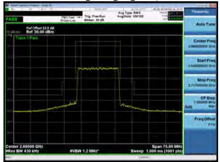
Band 41_16QAM_20M_RB100,0
