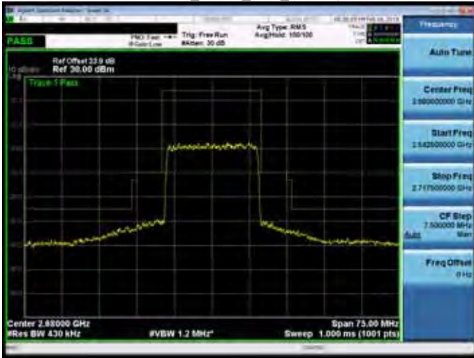
Band 41_16QAM_20M_RB1,0
