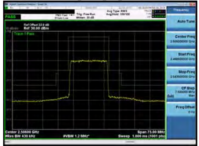
Band 41_16QAM_20M_RB1,0
