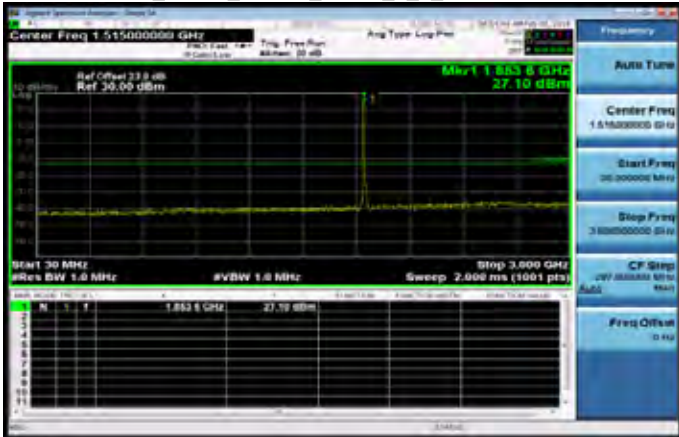
30MHz-3GHz_Band2_15MHz_QPSK_1_0_LowCH18675-1857.5
