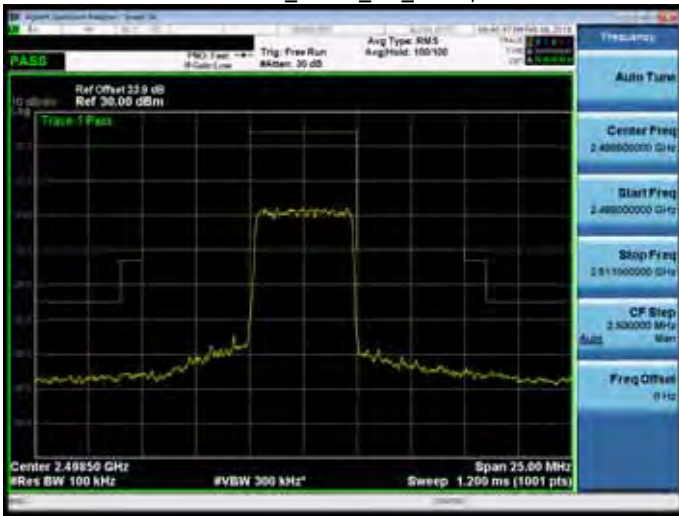
Band 41_QPSK_5M_RB1,0
