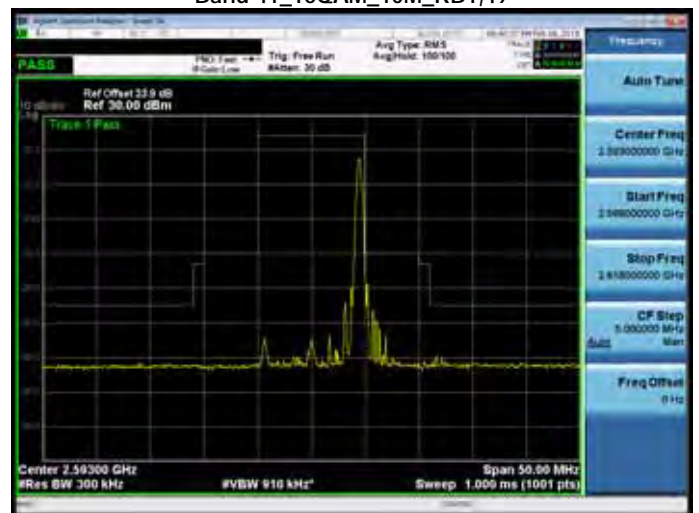
Band 41_16QAM_10M_RB1,49
