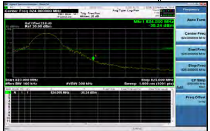
Part 90_Band26_10MHz_QPSK_1_49_HighCH26740
