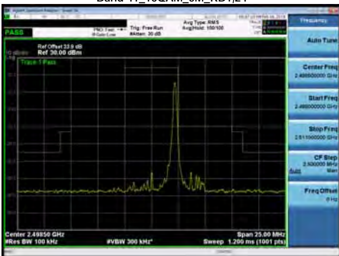
Band 41_16QAM_5M_RB1,24
