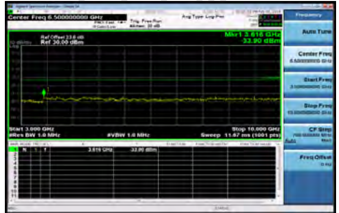
3GHz-10GHz_Band12_10MHz_QPSK_1_0_MidCH23095-707.5
