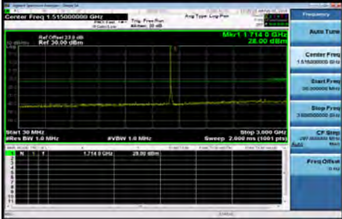
30MHz~3GHz_Band4_15MHz_QPSK_1_0_LowCH20025-1717.5
