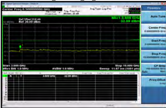
3GHz~10GHz_WCDMA_B5_LowCH4132-826.4
