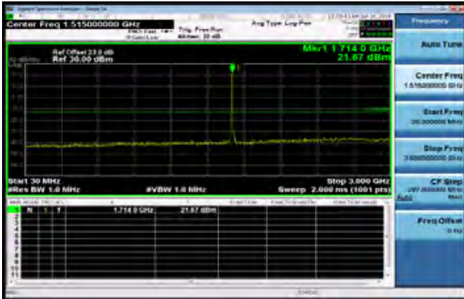
30MHz~3GHz_HSUPA_B4_LowCH1312-1712.4
