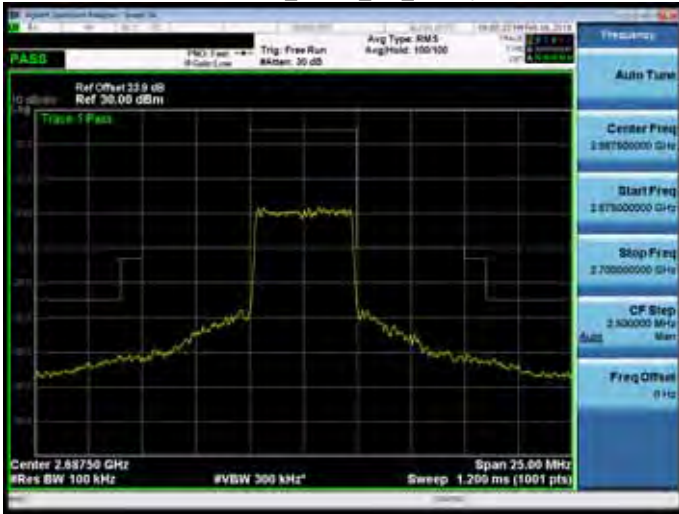
Band 41_16QAM_5M_RB1,0
