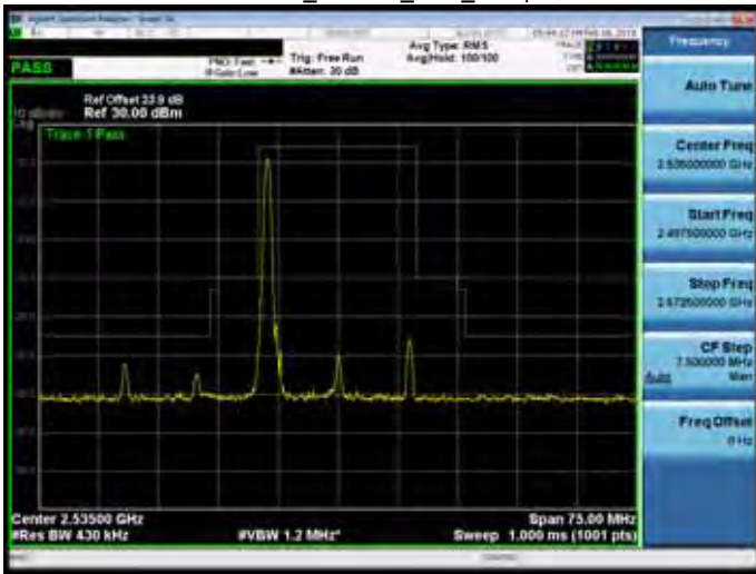
Band 7_16QAM_20M_RB1,99
