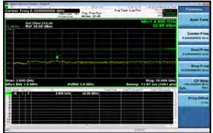
3GHz-10GHz_Band5_1_4MHz_QPSK_1_0_MidCH20525-836.5
