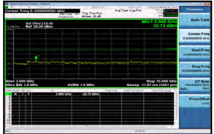
3GHz~10GHz_Band5_3MHz_QPSK_1_0_MidCH20525-836.5
