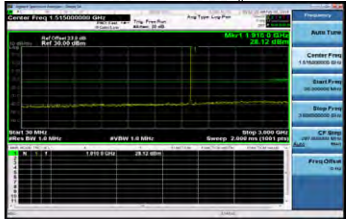
30MHz-3GHz_Band2_1_4MHz_QPSK_1_0_HighCH19193-1909.3
