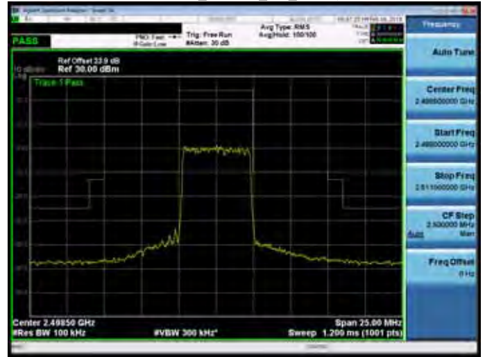
Band 41_16QAM_5M_RB1,0
