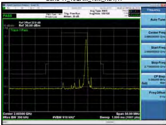
Band 41_16QAM_10M_RB1,49
