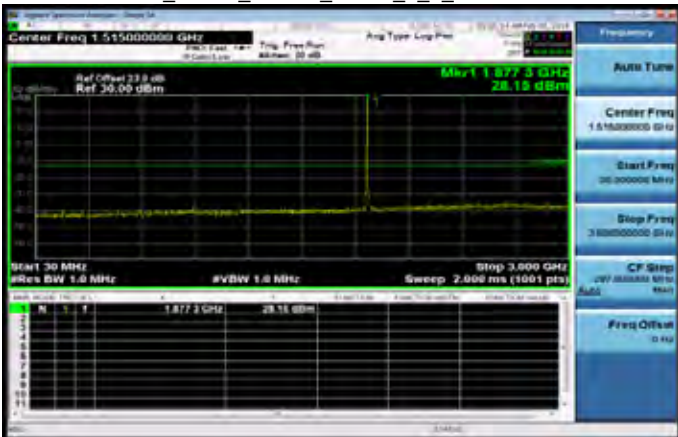
30MHz-3GHz_Band2_10MHz_QPSK_1_0_MidCH18900-1880
