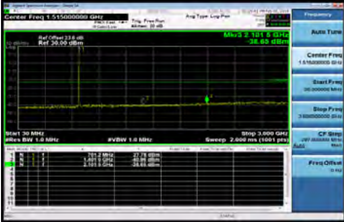
30MHz-3GHz_Band12_3MHz_QPSK_1_0_LowCH23025-700.5
