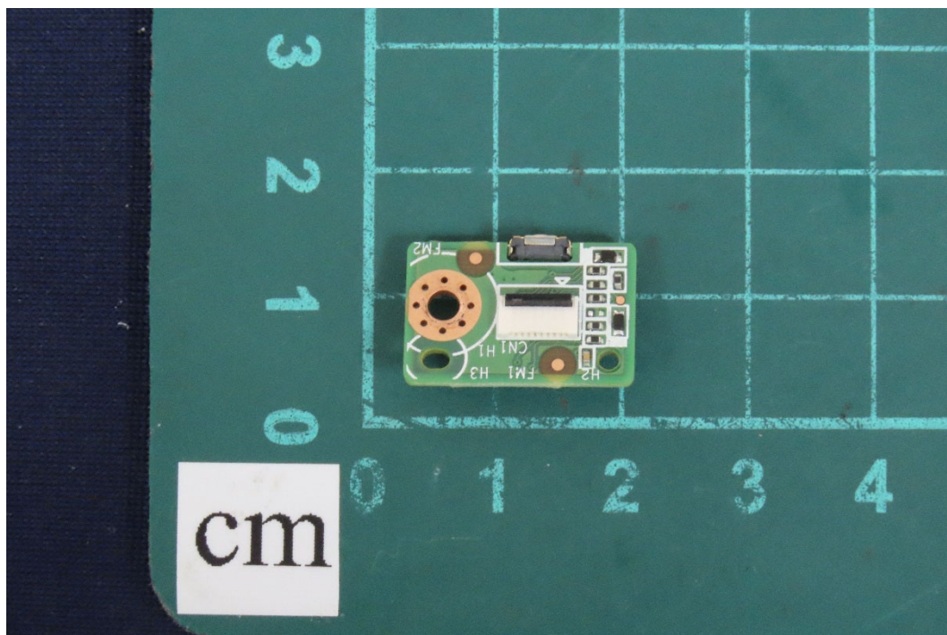
(25) EUT Photo
