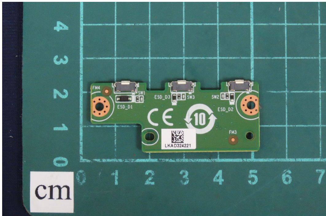
(34) EUT Photo
