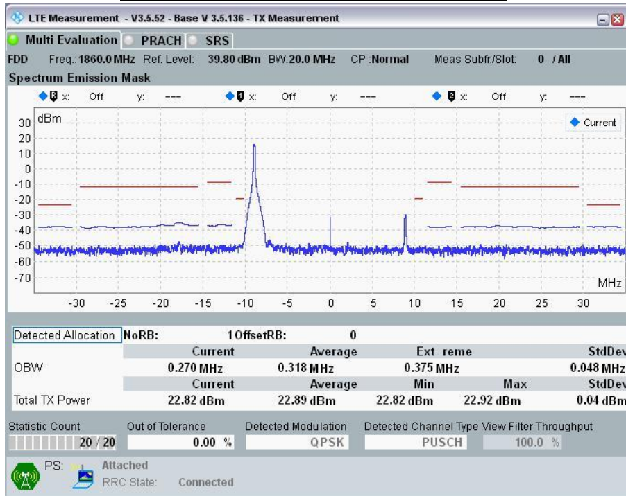
20MHz Band Width: Ch 18700, RB Size=1; RB Offset = 0
