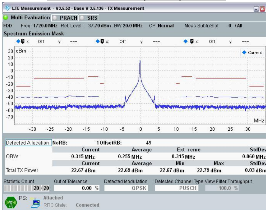
20MHz Band Width: Ch 20050, RB Size=1; RB Offset = 49
