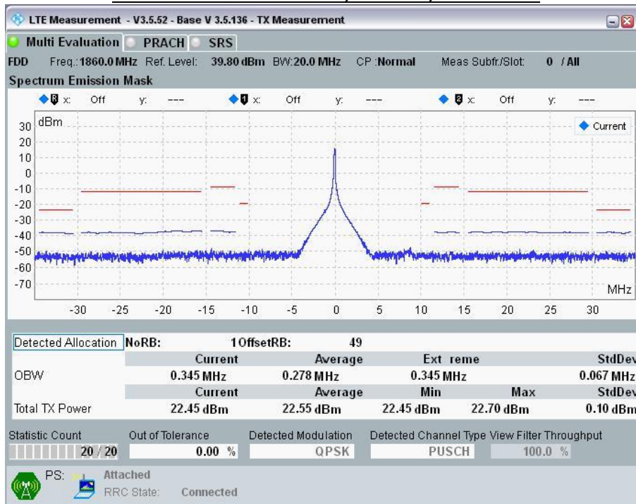
20MHz Band Width: Ch 18700, RB Size=1; RB Offset = 49
