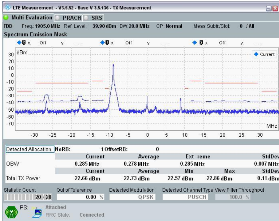
20MHz Band Width: Ch 26590, RB Size = 1; RB Offset = 0
