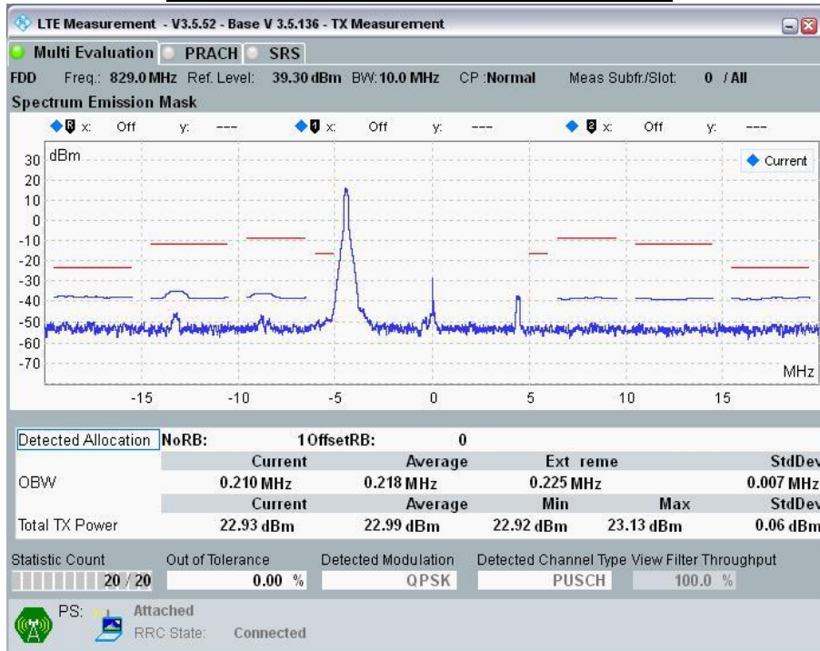
10MHz Band Width: Ch 20450, RB Size=1; RB Offset = 0
