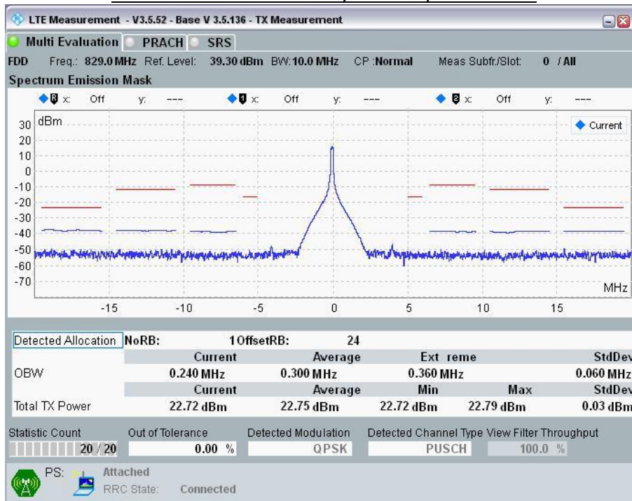
10MHz Band Width: Ch 20450, RB Size=1; RB Offset = 24
