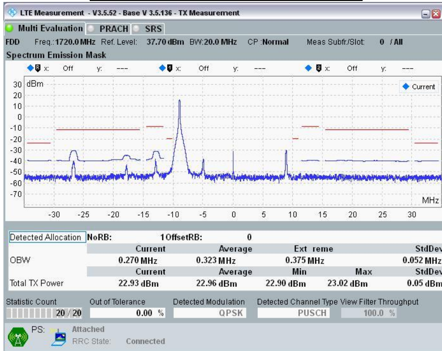
20MHz Band Width: Ch 20050, RB Size=1; RB Offset = 0
