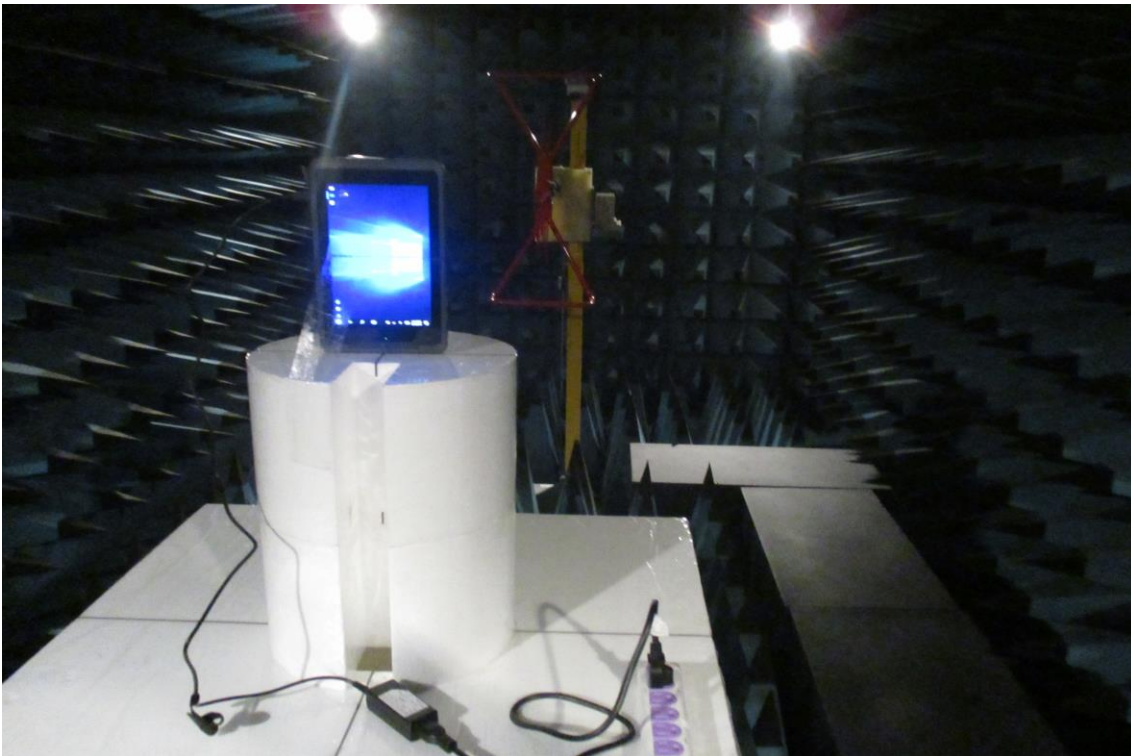
LTE Band 5
