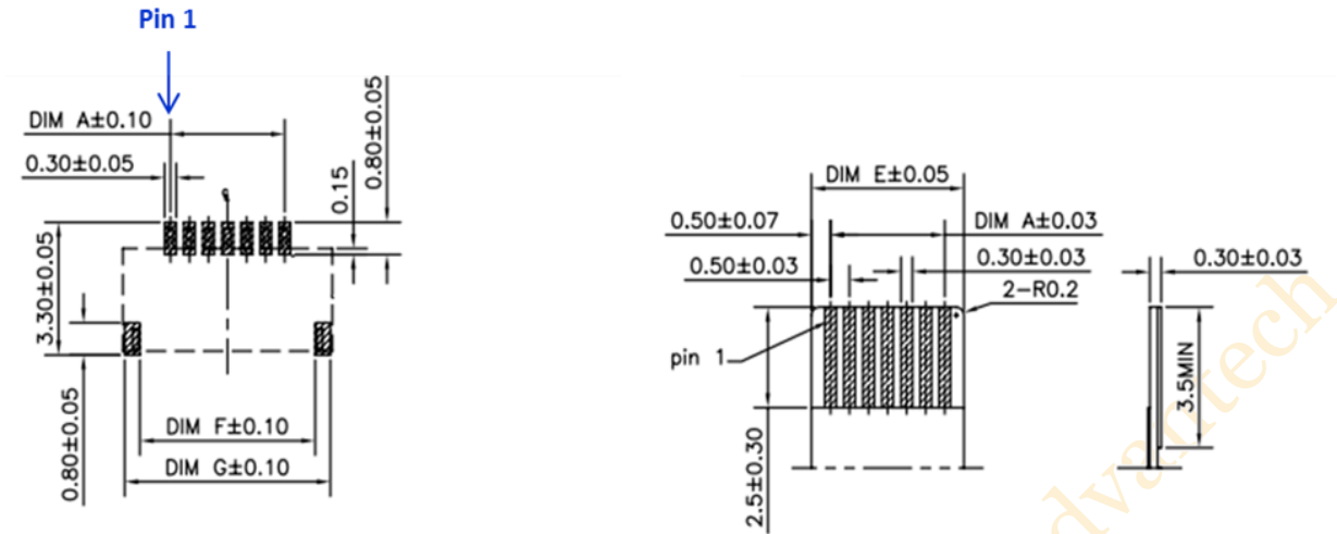
Figure 9 Module FPC Connection Footprint (Button Contact)
