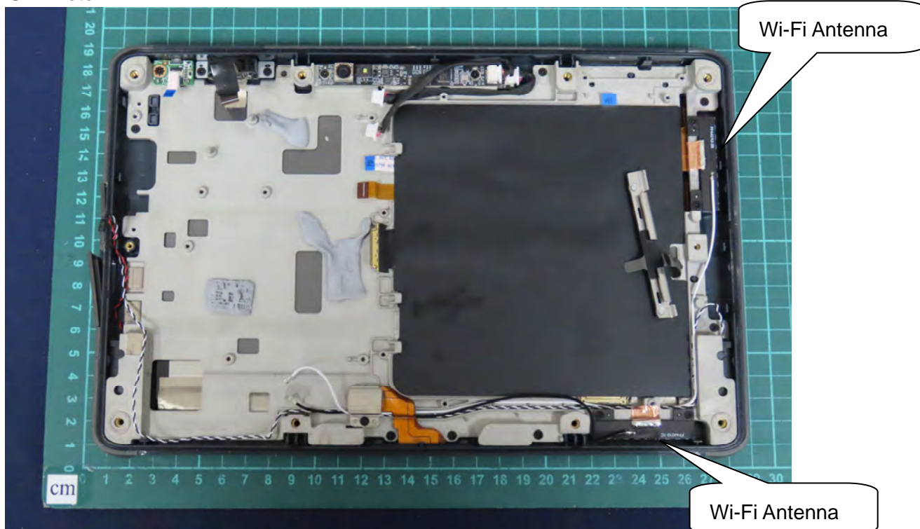
(28) EUT Photo
