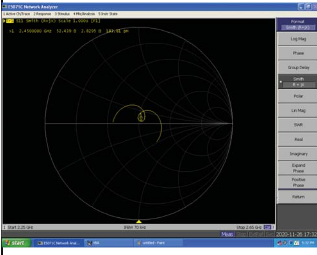
Impedance Test-Head
