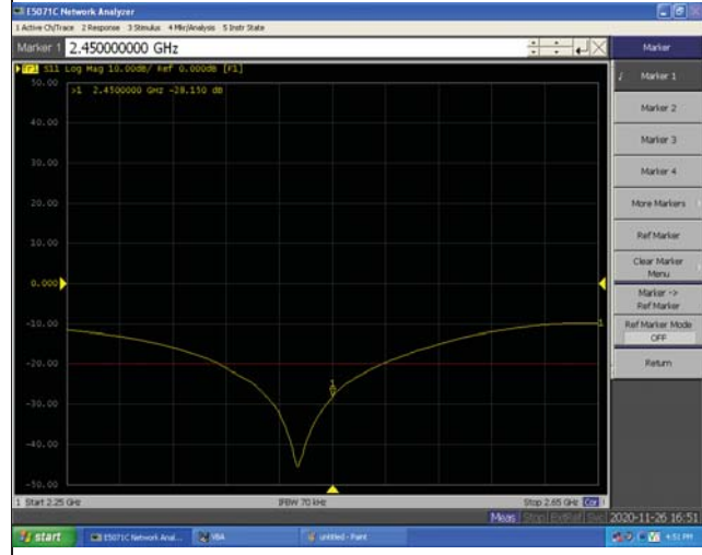
Return Loss-Head
